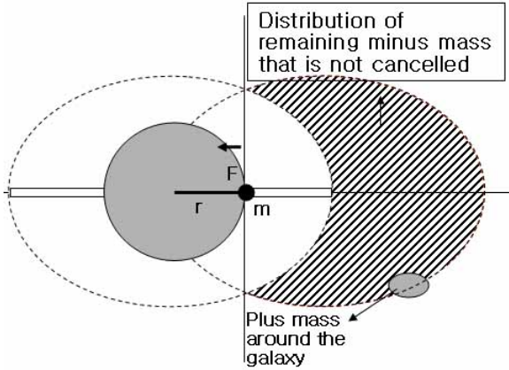
Figure 11: Equal to the degree of gravity that is applied on the equally distributed plus mass within the radius r of the left side. The gravitational effect from minus mass, which functions at mass m is equal to the gravitational effect from plus mass within radius r .
