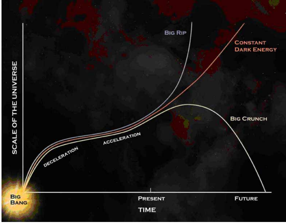
Figure 14: Deceleration and acceleration of the universe
