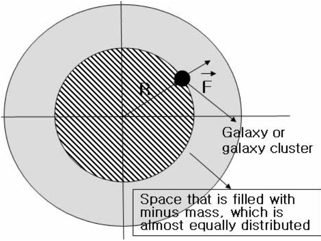
Figure 6: Expansion of the universe by minus mass distribution. The force, which is applied to the galaxy and galaxy cluster and located within radius R from the center of a 3-dimensional space, when assuming equal distribution of minus mass from repulsive effects between minus masses across space is valid.
