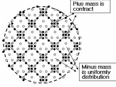
Figure 18: Contraction of plus mass
