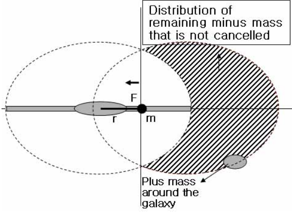
Figure 10: Effective minus mass. The minus mass distribution, where gravity is applied without cancellation of the oblique field located on the right side.
