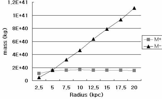
Figure 13: Distribution of plus mass and minus mass on NGC6503. The distribution of the galaxy mass, which is can be observed, is mostly in the galaxy nuclei, while the effects of minus mass, which is distributed over the outside of the galaxy, increases with the ratio of distance r.
