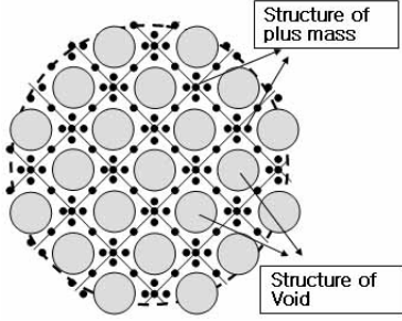
Figure 19: Structure of universe
