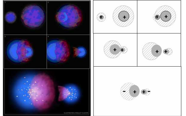
Figure 21: Collision of bullet cluster. We can see that general matters are close to each other, and dark matters are on the far side.
