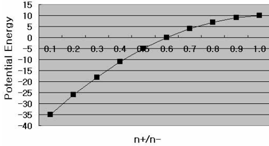
Figure 15: Potential energy from ratio of minus mass and plus mass
