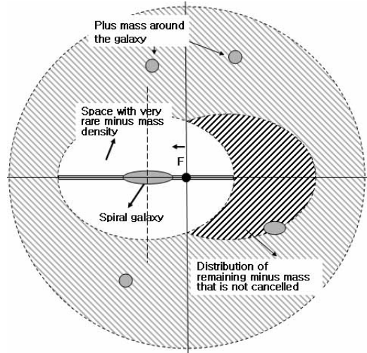
Figure 5: Minus mass effect on arms of galaxy. The actual observed spiral galaxy is on the left. Since repulsive effects occur between minus masses in Newtons dynamics, minus masses will be distributed all over space because it cannot form large mass structures like stars. Minus mass within the galaxy is cancelled out by attraction from large plus mass during the galaxy formation process. Furthermore, the space, other than the galaxy, will maintain the distribution state of minus mass.
