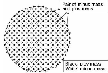
Figure 16: Pair creation
