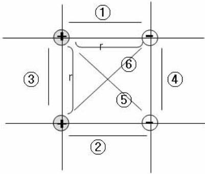
Figure 8: Arranges 2 when 2 pairs of minus and plus masses exist
