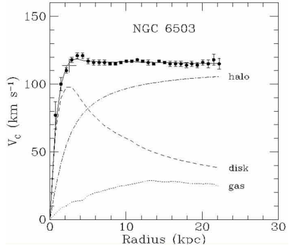
Figure 12: Revolution velocity of NGC 6503
