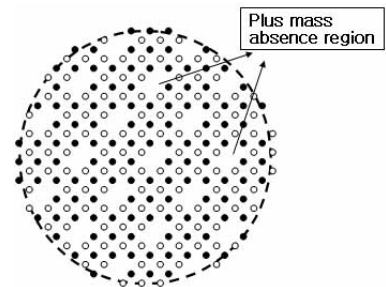
Figure 17: Plus mass absence region by pair annihilation or gravity effect
