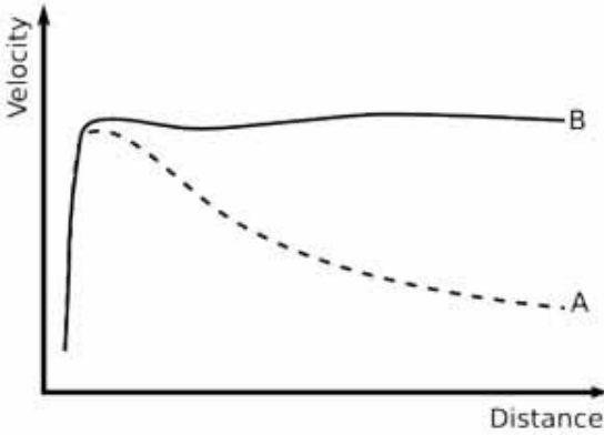
Figure 4: Revolution velocity of galaxy. The revolution velocity through the total quantity of matter that can be observed is A, while the actual observed value is B.
