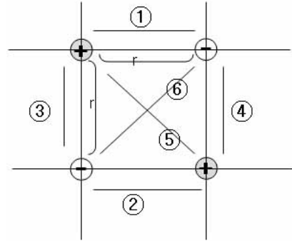
Figure 7: Arranges 1 when 2 pairs of minus and plus masses exist
