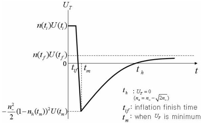
Figure 20: Changes in potential energy over time
