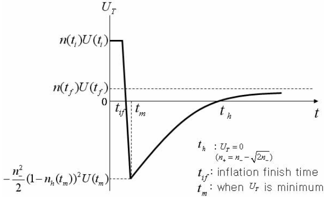
Figure 21: Changes in potential energy over time
