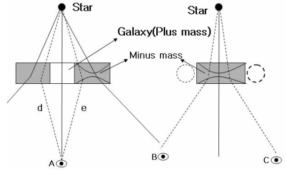
Figure 10: Concave Gravitational lensing effect. The left side is the Gravitational lensing effect that occurs when the galaxy is surrounded by minus mass and the right side is Gravitational lensing effect that occurs when plus mass exists alone
