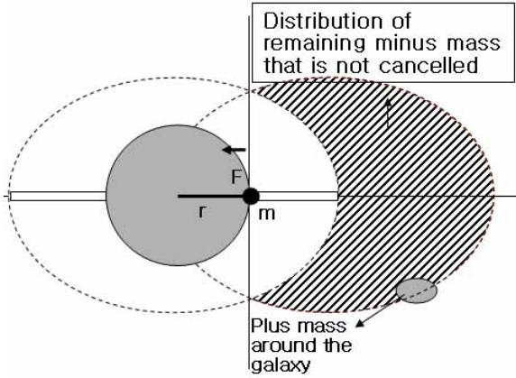
Figure 12: Equal to the degree of gravity that is applied on the equally distributed plus mass within the radius r of the left side. The gravitational effect from minus mass, which functions at mass m is equal to the gravitational effect from plus mass within radius r .
