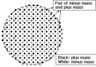
Figure 17: Pair creation
