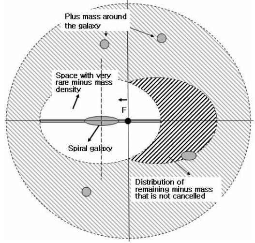
Figure 6: Minus mass effect on arms of galaxy. The actual observed spiral galaxy is on the left. Since repulsive effects occur between minus masses in Newtons dynamics, minus masses will be distributed all over space because it cannot form large mass structures like stars. Minus mass within the galaxy is cancelled out by attraction from large plus mass during the galaxy formation process. Furthermore, the space, other than the galaxy, will maintain the distribution state of minus mass.
