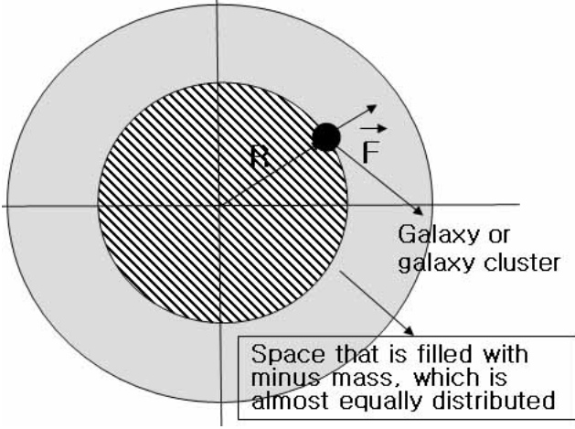
Figure 7: Expansion of the universe by minus mass distribution. The force, which is applied to the galaxy and galaxy cluster and located within radius R from the center of a 3-dimensional space, when assuming equal distribution of minus mass from repulsive effects between minus masses across space is valid.
