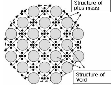
Figure 20: Structure of universe
