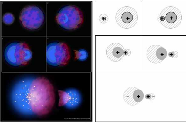
Figure 22: Collision of bullet cluster. We can see that general matters are close to each other, and dark matters are on the far side.
