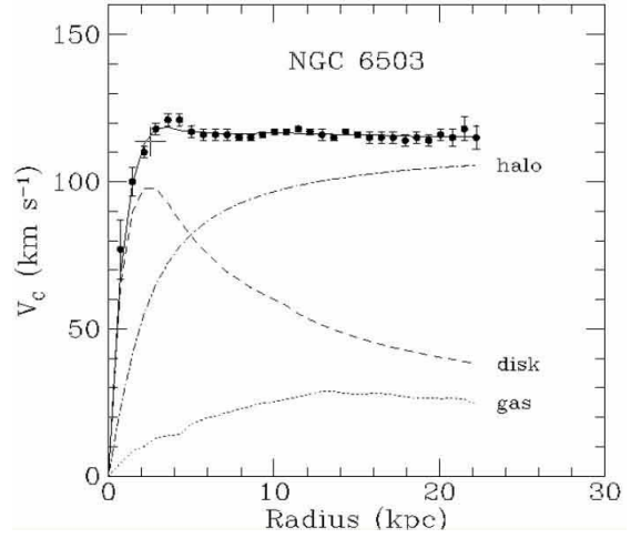
Figure 13: Revolution velocity of NGC 6503
