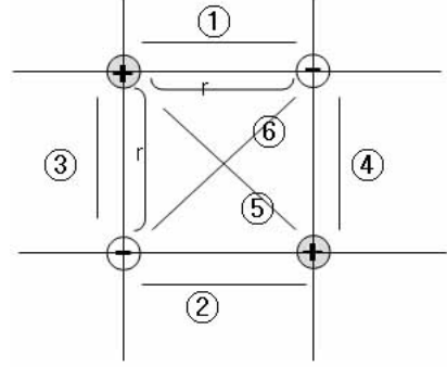
Figure 8: Arranges 1 when 2 pairs of minus and plus masses exist
