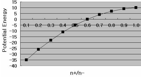
Figure 16: Potential energy from ratio of minus mass and plus mass
