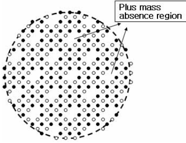
Figure 18: Plus mass absence region by pair annihilation or gravity effect
