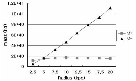
Figure 14: Distribution of plus mass and minus mass on NGC6503. The distribution of the galaxy mass, which is can be observed, is mostly in the galaxy nuclei, while the effects of minus mass, which is distributed over the outside of the galaxy, increases with the ratio of distance r .
