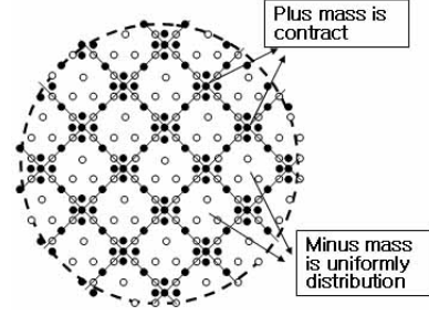
Figure 19: Contraction of plus mass
