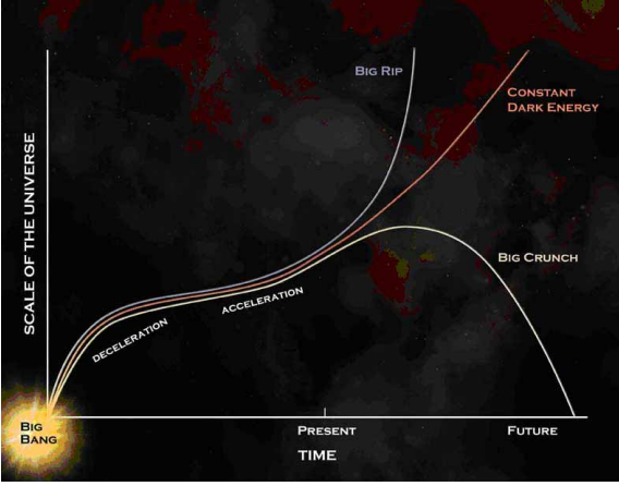
Figure 15: Deceleration and acceleration of the universe
