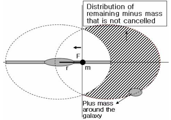
Figure 11: Effective minus mass. The minus mass distribution, where gravity is applied without cancellation of the oblique field located on the right side.
