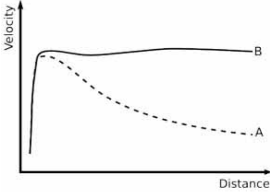
Figure 5: Revolution velocity of galaxy. The revolution velocity through the total quantity of matter that can be observed is A, while the actual observed value is B.
