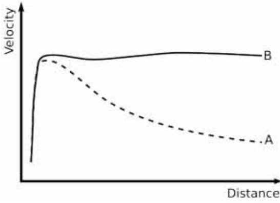
Figure 6: Revolution velocity of galaxy. The revolution velocity through the total quantity of matter that can be observed is A, while the actual observed value is B.
