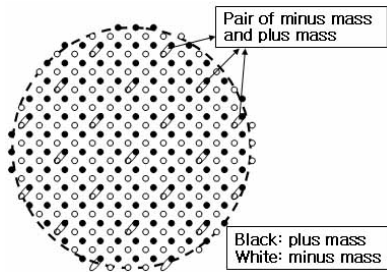
Figure 18: Pair creation
