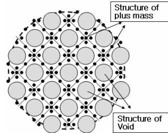
Figure 21: Structure of universe
