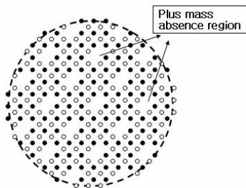
Figure 19: Plus mass absence region by pair annihilation or gravity effect
