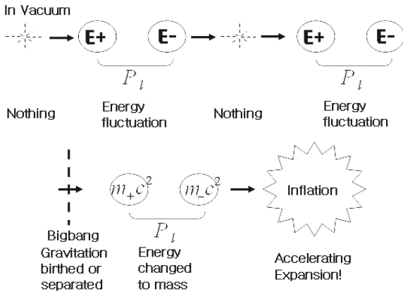
Figure 22: Concept of Bigbang and Inflation
