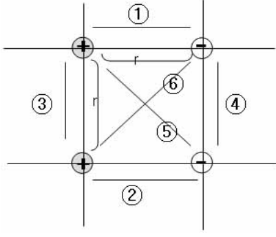
Figure 10: Arranges 2 when 2 pairs of minus and plus masses exist
