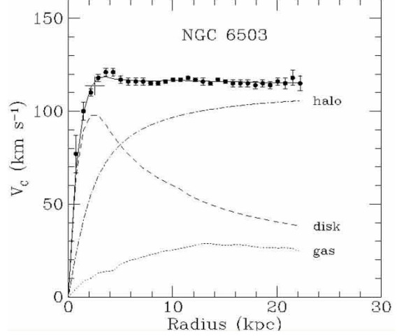
Figure 14: Revolution velocity of NGC 6503
