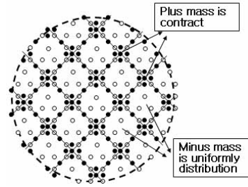
Figure 20: Contraction of plus mass
