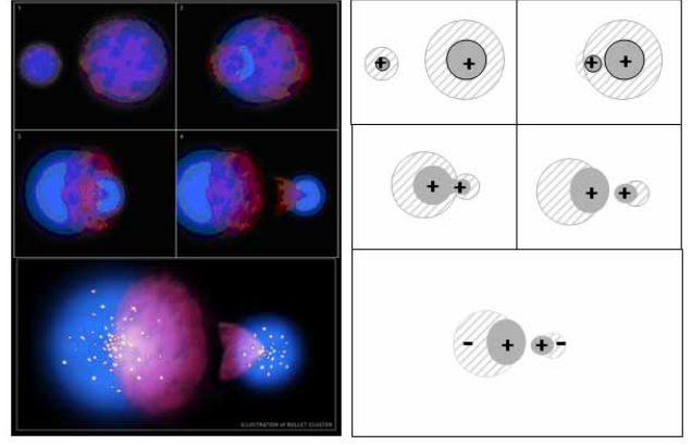
Figure 24: Collision of bullet cluster. We can see that general matters(red color) are close to each other, and dark matters(blue color) are on the far side.
