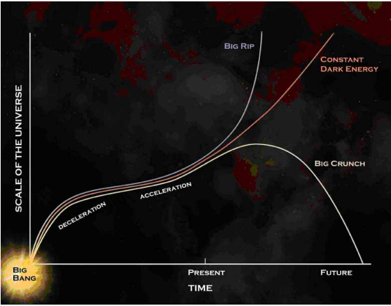
Figure 16: Deceleration and acceleration of the universe
