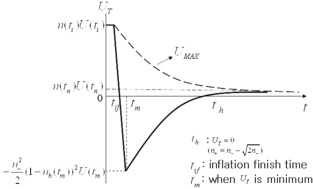
Figure 23: Changes in universe's potential energy over time
