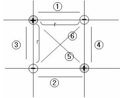
Figure 6: Arranges 1- when 2 pairs of negative and positive masses exist
