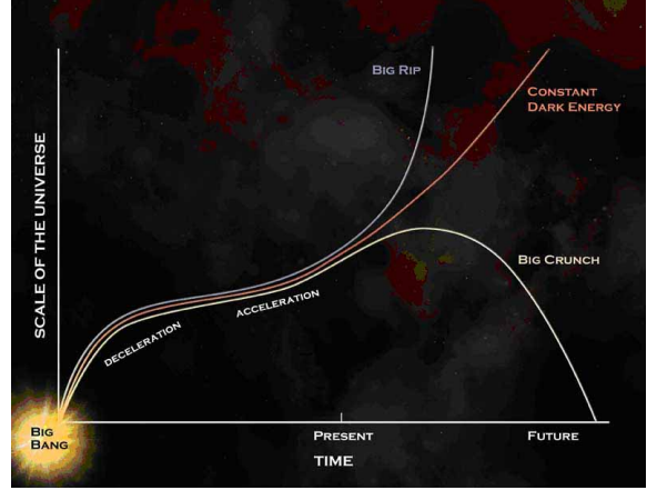
Figure 8: Decelerating expansion and accelerating expansion of the universe
