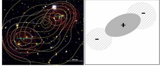
Figure 21: MACS J0025.4-1222 Cluster. We can see that general matters(yellow color) are close to each other(center), and dark matters(red color) are on the far side. [19]
