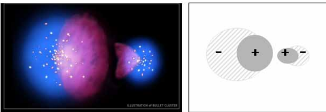
Figure 20: Collision of Bullet Cluster. We can see that general matters(red color) are close to each other, and dark matters(blue color) are on the far side. [18]
