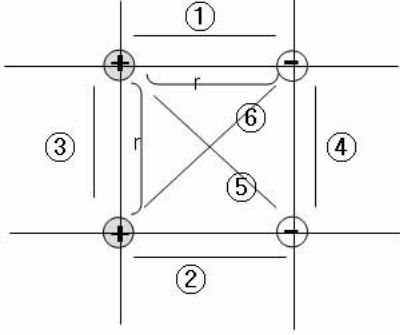
Figure 7: Arranges 2- when 2 pairs of negative and positive masses exist
