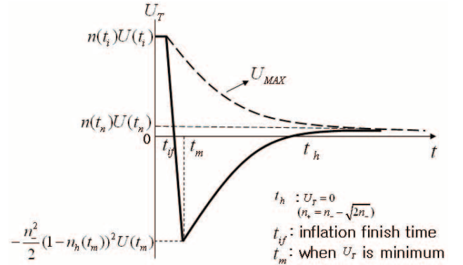
Figure 18: Changes in universe's potential energy over time
