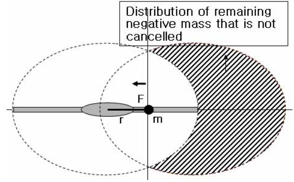
Figure 15: Effective negative mass. The negative mass distribution, where gravity is applied without cancellation of the oblique field located on the right side.
