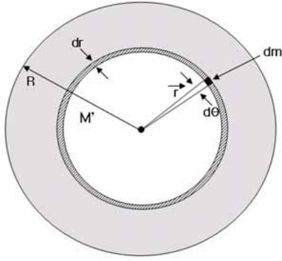
Figure 10: Gravitational self-energy
