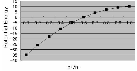
Figure 9: Potential energy from ratio of negative mass and positive mass
