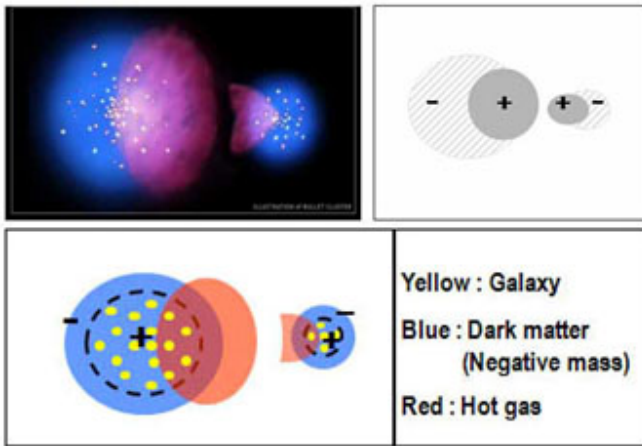
Figure 22: Collision of Bullet Cluster. We can see that general matters(red color) are close to each other, and dark matters(blue color) are on the far side. [20]
