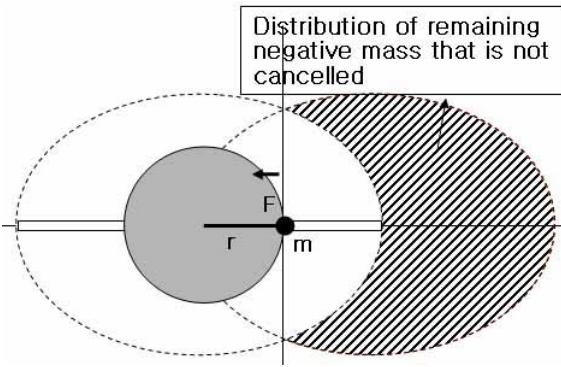
Figure 16: Equal to the degree of gravity that is applied on the equally distributed positive mass within the radius r of the left side. The gravitational effect from negative mass, which functions at mass m is equal to the gravitational effect from positive mass within radius r .
