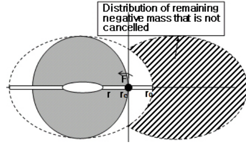
Figure 19: Spherical approximation method is valid to the short axis radius.
