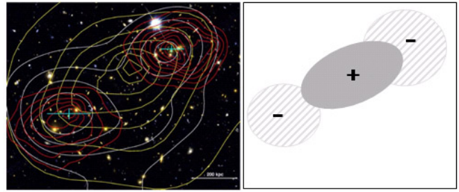
Figure 23: MACS J0025.4-1222 Cluster. We can see that general matters(yellow color) are close to each other(center), and dark matters(red color) are on the far side. [21]
