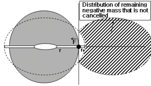
Figure 20: Spherical approximation method has a more mass effect above the short axis radius.
