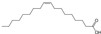
Figure 3.5: Oleic acid
