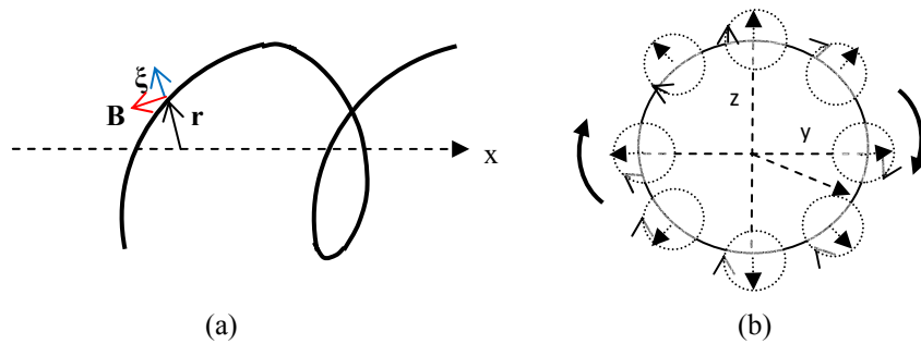
(a) shows that the field of the EM wave moves on a helical path with the electrical field always perpendicular to the direction of propagation but parallel to the radius vector while the magnetic field is orthogonal to both electric and the direction of propagation. (b) gives the transverse cross sectional view of the helical wave. Note that the electric field (magnetic field not shown) is always directed outward in line with the radius vector.
