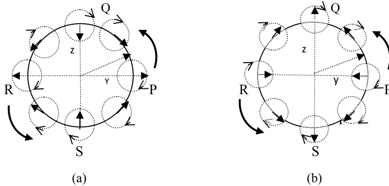
(a) shows the case where the rotation of the helical wave is in the anti-clockwise direction while the electric field rotates in the opposite direction. The field has positive component \xi_y at P on the y-axis and becomes -\xi_z at Q, then -\xi_y at R and \xi_z at S. (b) represents the case with the same direction of rotation but with the phase of of the electric vector differing from that of case (a) by \pi .
