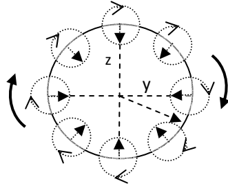
The figure gives the view of the EM wave in the direction of the progression .Here the phase of the electric field denoted by the arrow in the epicycle differs from that of the radius vector by \pi .
