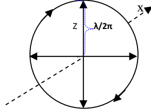
The figure represents transverse view of a propagating electromagnetic wave. The vertical and the horizontal lines stand for two perpendicular oscillations having phase difference of \frac{1}{2}\pi . Here the circular velocity is taken as c .
