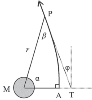
Fig. 1: Light deflection in a radially-dependent index of refraction
