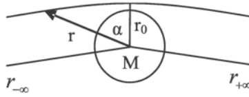
Fig. 2: Light deflection in a gravitational field
