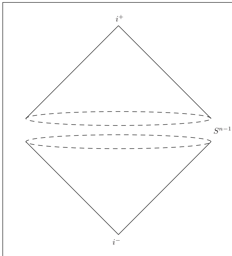
Figure 5: Chronological boundary for \mathbb{L}^{n+1} - Figure. 2 from [5]
