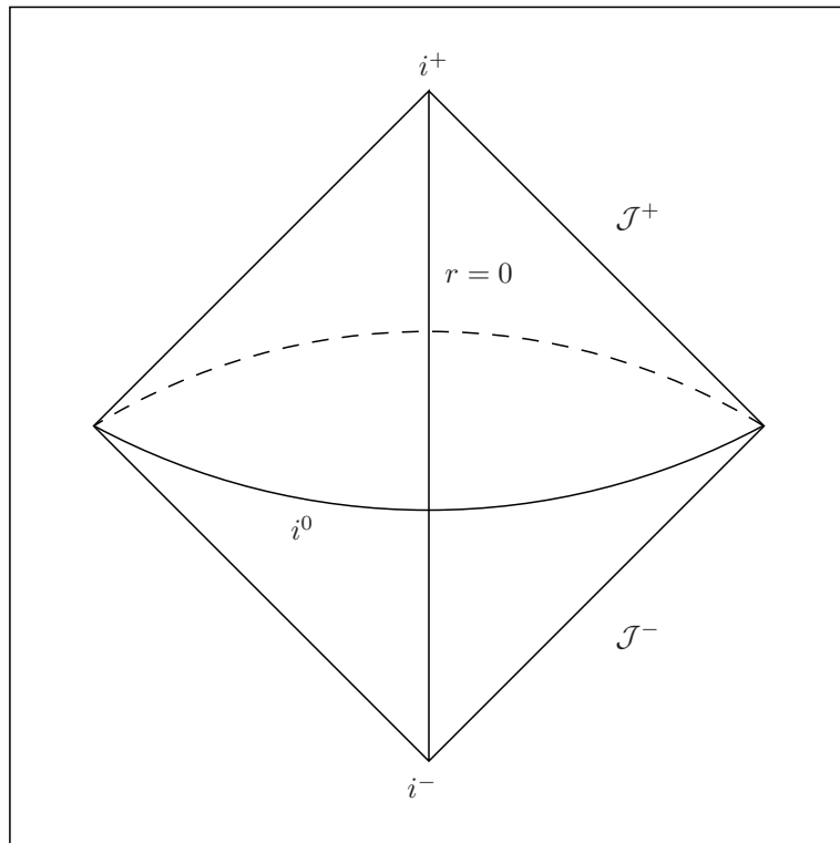
Figure 4: Conformal infinity of Minkowski space from [4, p. 178]. The meaning of this picture is quite different from the one in Fig. 3, where the points i^0, i^+, i^- are identified. The 2-sphere indicated in the middle of this picture is just one point i^0 and not the true 2-sphere of Fig. 3
