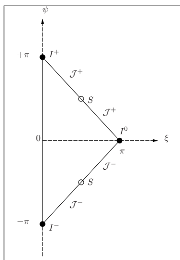
Figure 1: The “Penrose diagram” of Minkowski space.
