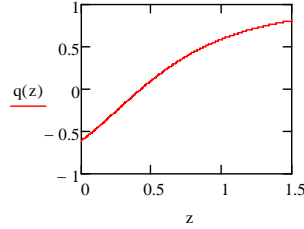
Fig. 1: Reacceleration of the universe based on Beckwith 7 (note that q < 0 if z < .423 )
