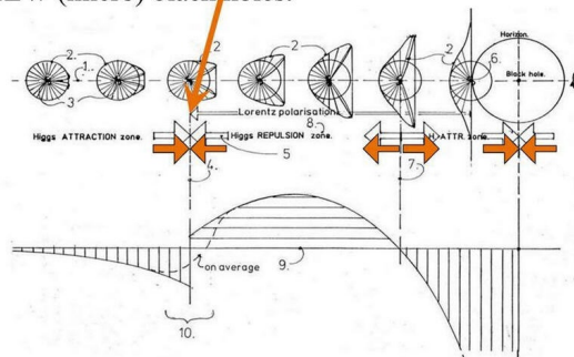
Figure 10, Comparison with splitting and pairing Micro black holes inside Planetary nebula, and the formation of comet nuclei like the Hyperion icy nucleus.
