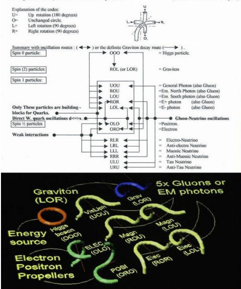
The alternative standard model with some 3-D examples of different particles? Figure 7, the alternative standard model ref. [5]
