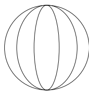
Fig 4: Sectoral nodes in spherical harmonics.
