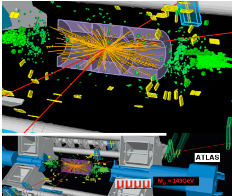
Here is an image of an ATLAS Golden Channel candidate mid-mass ● Higgs event:
