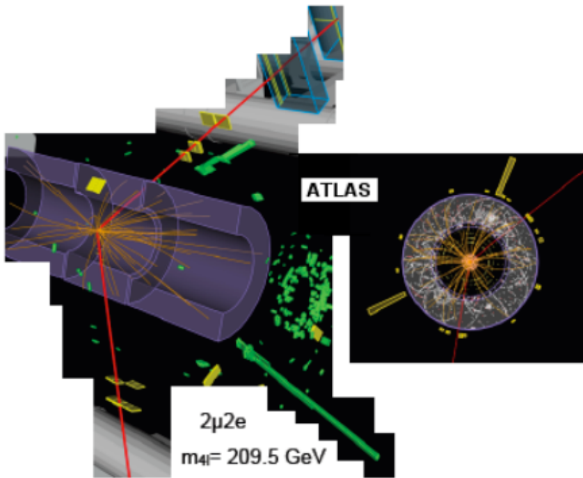
Here is an image of an ATLAS Golden Channel candidate mid-mass ● Higgs event:
