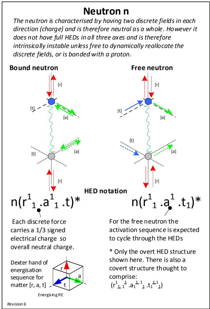
Figure 1: Proposed internal and external (discrete force) structures of the neutron.
