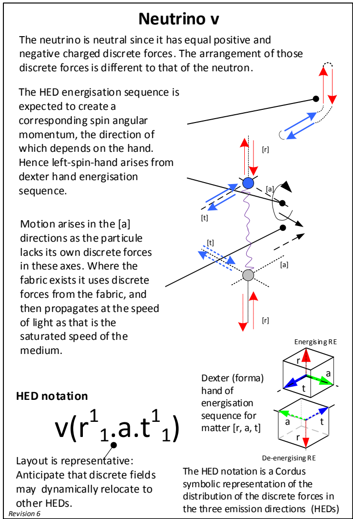
Figure 4: Predicted structure of the neutrino.
