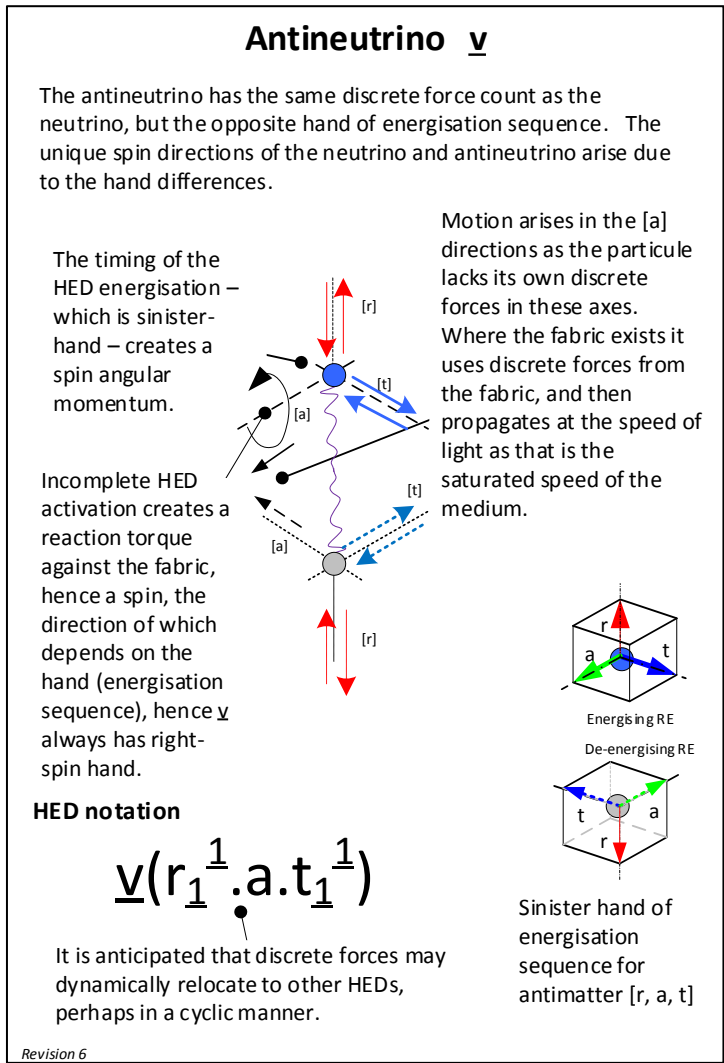
Figure 3: Predicted structure of the antineutrino.
