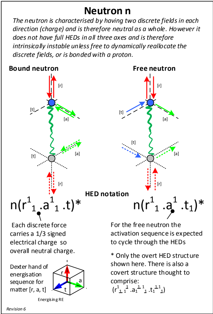
Figure 1: Proposed internal and external (discrete force) structures of the neutron. From [9] reproduced by permission.
