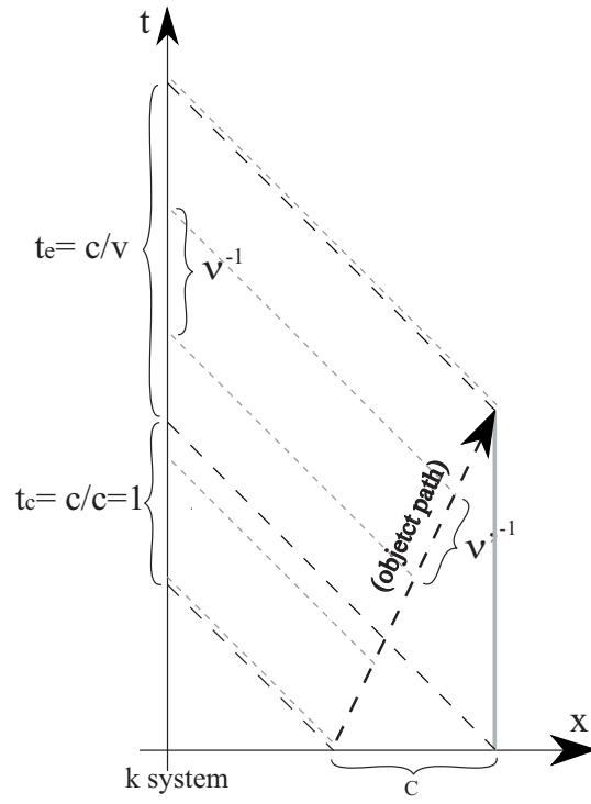
FIG. 6 Graphical explanation of Eq. (??) for \nu^+ .
