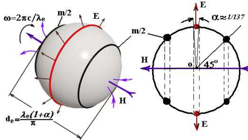
Figure 2. Schematic Model of the Electron
