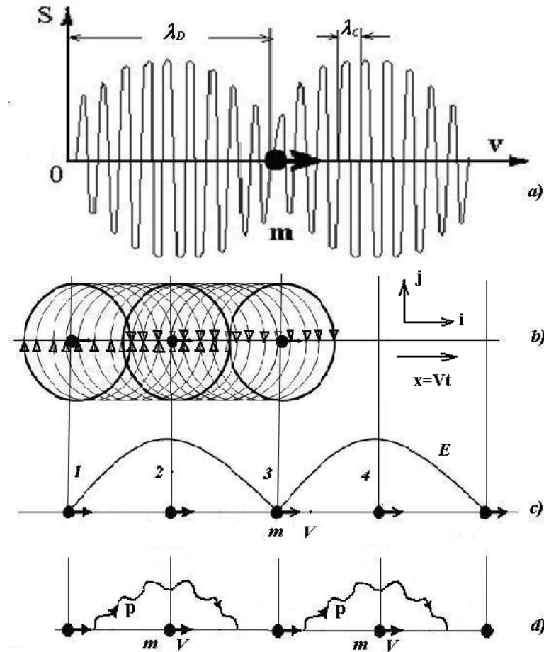
Fig. 3. De Broglie's wave illustration
