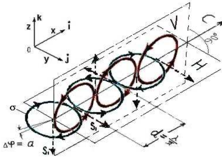
Figure 1. The Scheme of Quantum Wave-Packet
