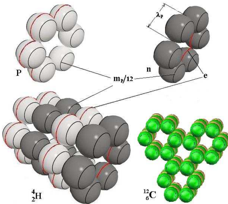
Figure 8 The schemas of proton, neutron, helium and carbon nucleuses
