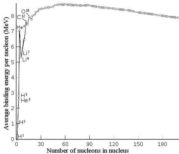
Figure 9. The curve of binding energy
