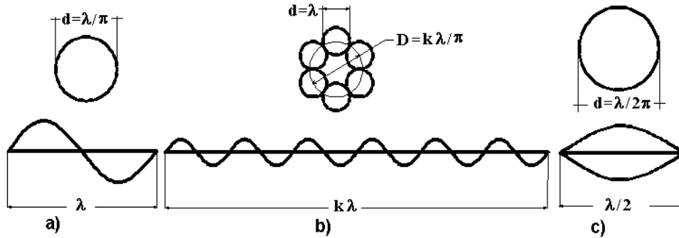
Figure 6. Possible kinds of QEF localisations
