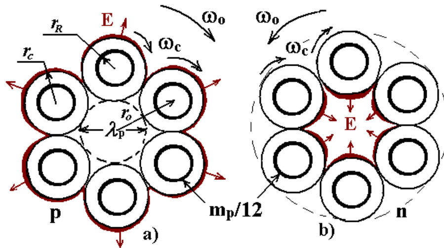
Figure 7. Scheme of the proton a), neutron b)
