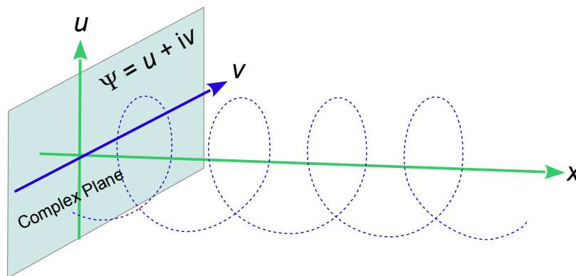
Figure 5: The abstract wavefunction (pure momentum state)
