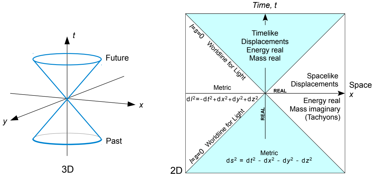
Figure 6: Minkowski spacetime
