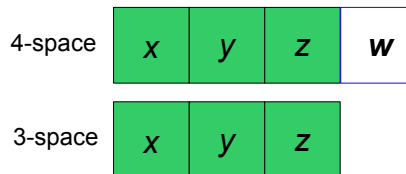
Figure 8: The spatial domain of quantum mechanics
