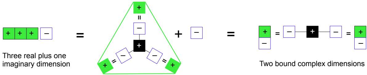
Figure 16: Spatial configurations of the 4-brane
