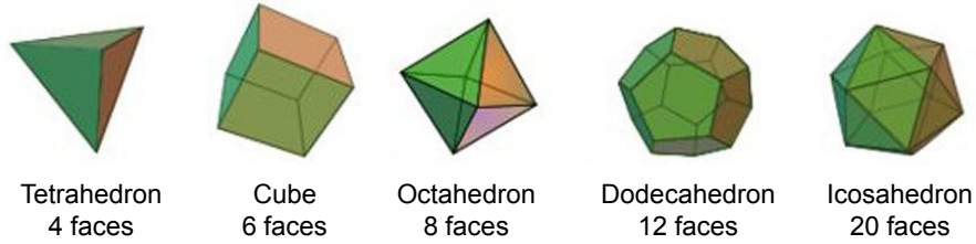
Figure 25: The five Platonic solids
