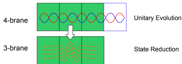
Figure 23: The action of the wavefunction
