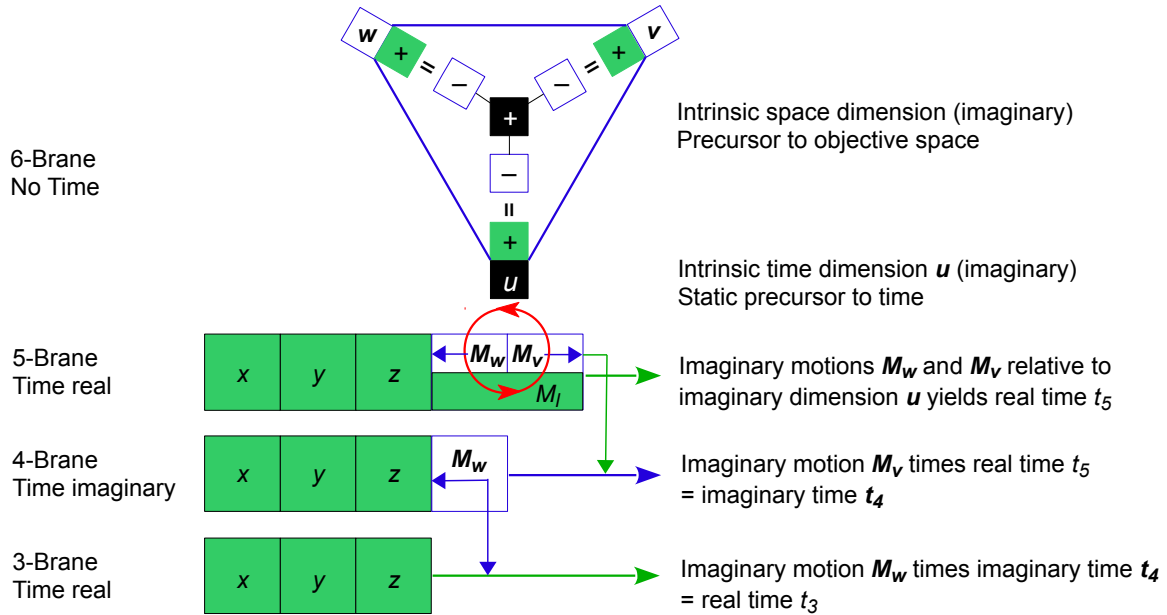
Figure 20: The genesis of time and energy
