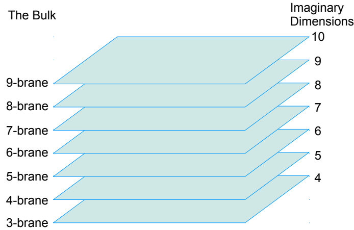
Figure 14: Interpenetrating spaces
