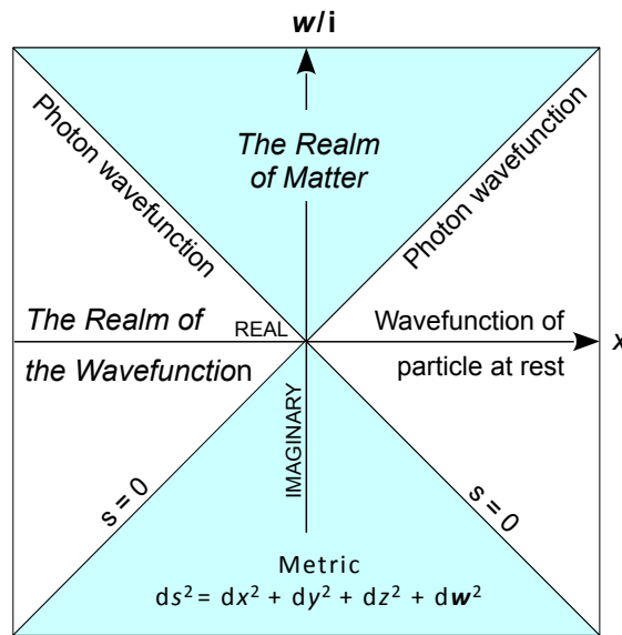
Figure 9: Minkowski 4-Space
