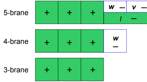
Figure 13: Spatial dimensions of the lower three branes
