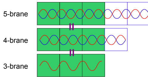
Figure 21: The unifying 5-dimensional wavefunction
