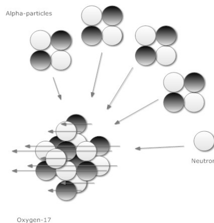
Figure 2: Oxygen-17
