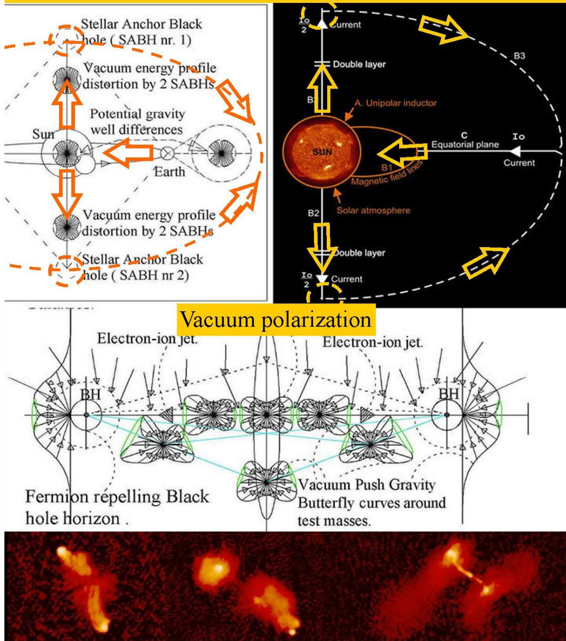
Figure: 15, Birkeland/ Alfvén circuit currents around stars and galaxies, are driven by new paradigm tandem black holes, each producing a global external excess of negative charged plasma and an internal positive charge plasma. The negative plasma is mainly accelerated as Birkeland Alfvén current circuits by the Casimir polarized vacuum (or Higgs polarized oscillations, according to Q-FFF Theory)
