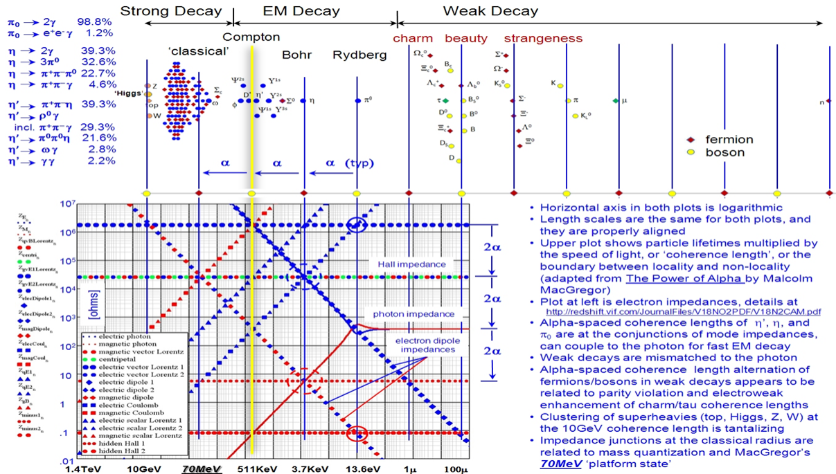
Fig. 1. Composite of 13.6eV photon [6] and background independent electron impedances [3], measured \pi_0 , \eta , and \eta' branching ratios, and unstable particle coherence lengths [7].
