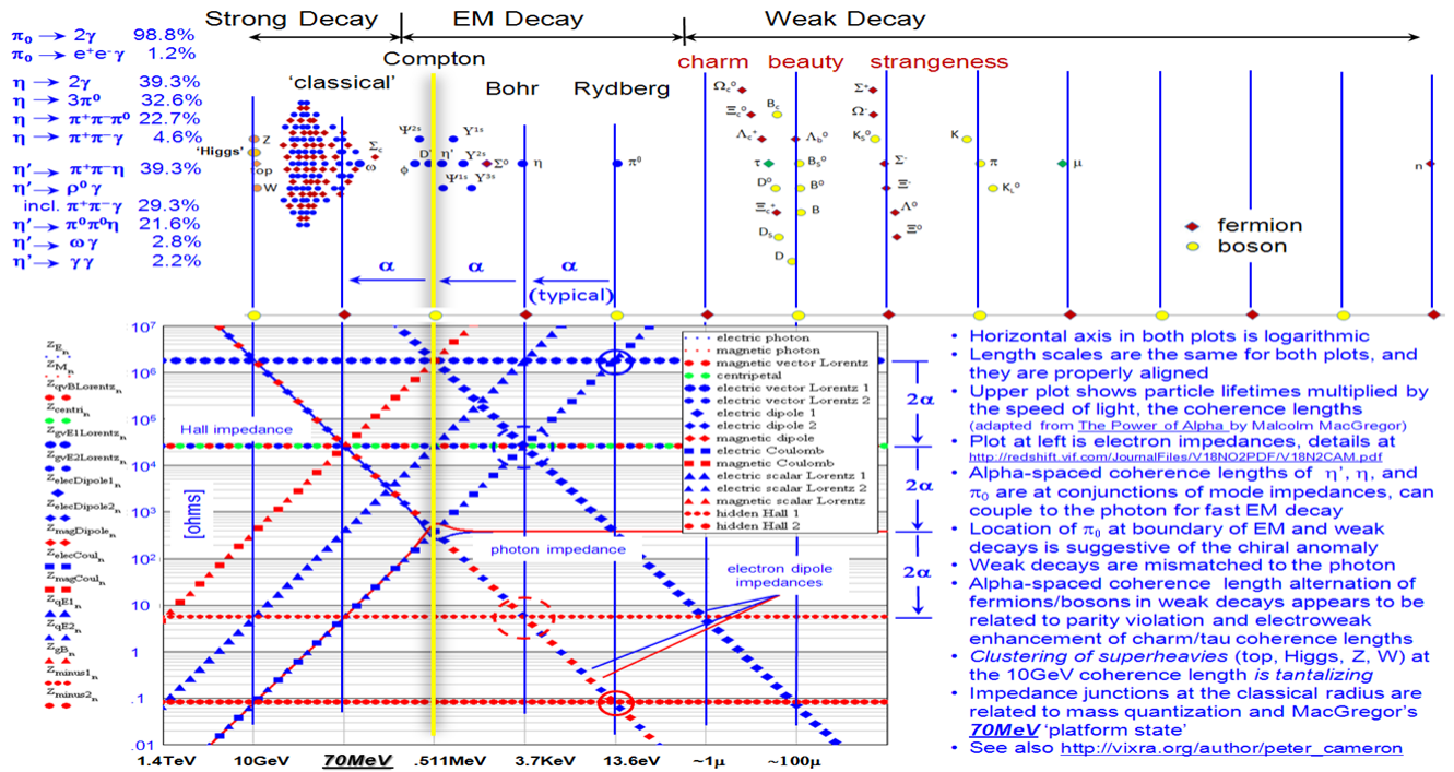
Fig. 1. Composite of 13.6eV photon [6] and background independent electron impedances [3], measured \pi_0 , \eta , and \eta' branching ratios, and unstable particle coherence lengths [7].
