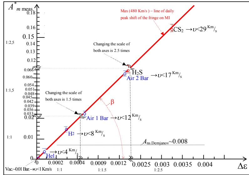
Fig.1. The dependence of the A_m(\Delta\epsilon) relative amplitude A_m of the interference fringe shift from the polarization contribution \Delta\epsilon = n^2 - 1 . particles in the total permittivity \epsilon = 1 + \Delta\epsilon light-carrying gaseous medium Michelson interferometer (MI), which have been discovered by me in 1968 [2] (here 1. – the relative permittivity of aether): Max (480 km/s) – line values of maximum shift of the fringe A_m on the daily trend of A_m(T) [2**] for different light-carrying medium MI, where T – local time (a local times T_m of occurrence of the maximum A_m in different months at a latitude of Obninsk are given in [2**]). Parameters of MI: the length of the rays in gases mediums: L_1 = L_2 = 7 m and length of wave \lambda = 6 \cdot 10^{-7} m, at normal pressure of gases (air humidity \sim 40\% ). Point Vac. corresponds to the rarefaction of the air 10^{-2} Bar., point Air 2 Bar. corresponds to the high pressure air. A_{ns} – average amplitude jitter noise interference fringe at the my experiments. The shift of the fringe on the MI with the helium medium (Hel.) is barely visible into the noise even at the "daily-peak shift of the fringe", and the shift of the fringe on the MI with the evacuated (Vac. \sim 10^{-2} Bar) light-bearing zones is practically not observed in the noise. Angle \beta is used in the analysis of formula (5).
