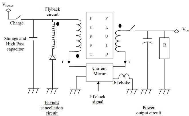
Figure 21 – The H-Field Cancellation Scheme (LHS circuit)
