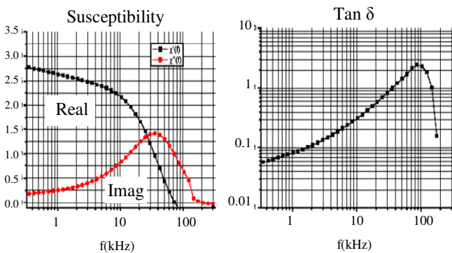
Figure 6 – Hysteresis loss in typical ferrofluid (Courtesy Sustech GmbH) LHS Bode plot in and out-phase components RHS: Power loss angle
