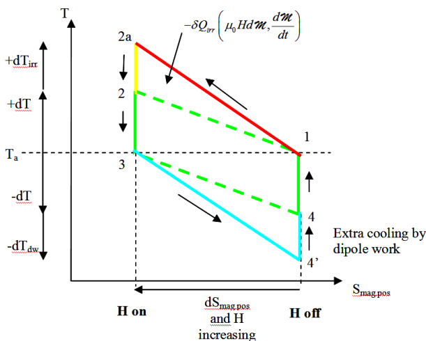
Figure 11 – Temperature- Positional Entropy Diagram for the micro-cycle
