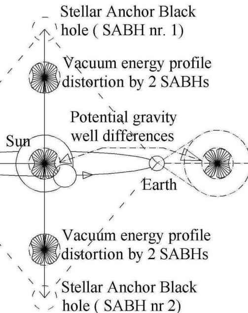
Figure 10. Stellar Anchor Black Holes (SABHs) and the Sun.
