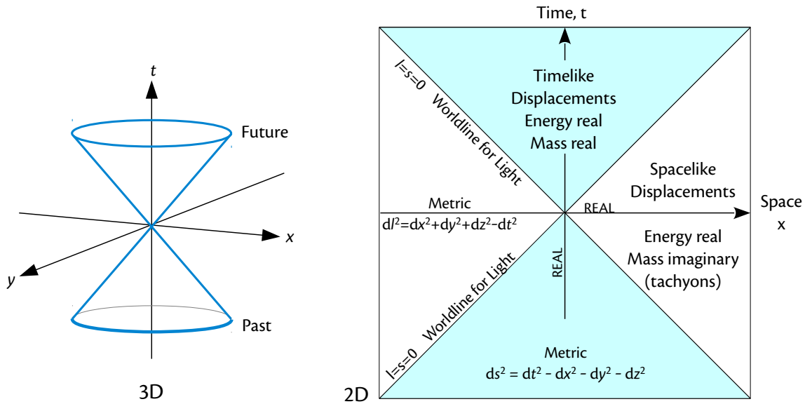
Figure 2 • Minkowski spacetime
