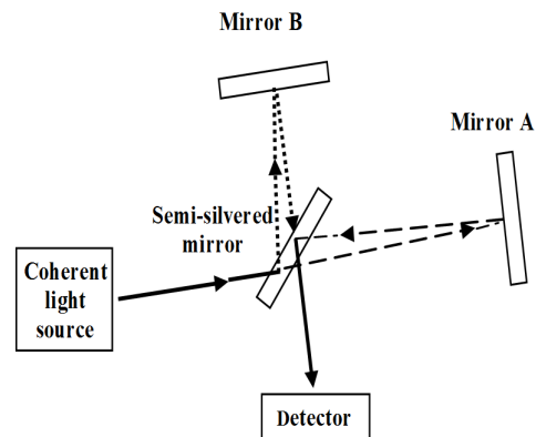
Fig. 1 The scheme of the Michelson interferometer
