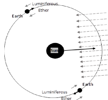
Fig. 2 The expected effect of the luminiferous ether on the speed of light
