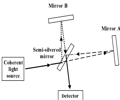
Fig. 1 The scheme of the Michelson interferometer
