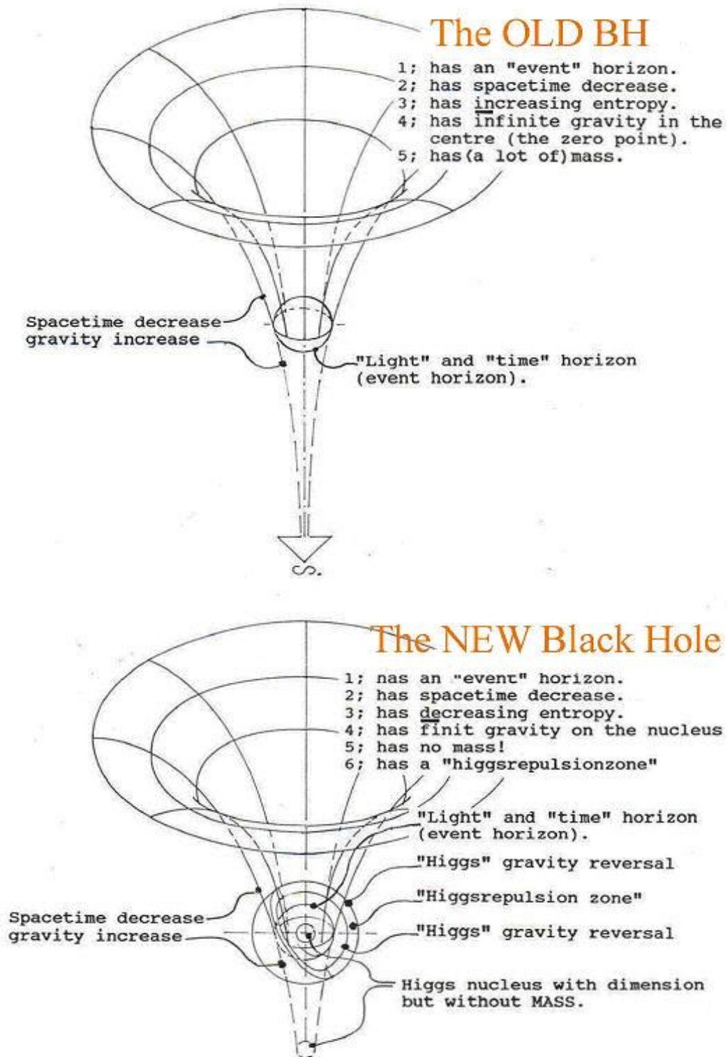
Figure 6, The difference between the old and new paradigm Black hole according to Quantum FFF Theory .
