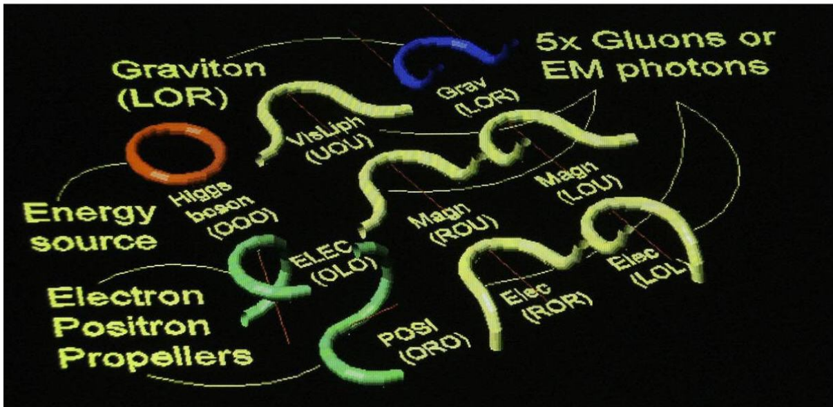
Figure 16, The particle zoo of single ELEMENTARY particles made out of ONE convertible Torus shaped Higgs particle, equipped with three hinges of 90 degree rotation.
