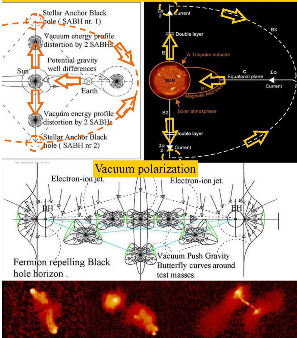
Figure: 10. Black hole propulsion and pairing principle of fig 8, seems to be the origin of dual Stellar or galaxy Anchor black holes (see figure 11) and even so called Birkeland /Alfven current circuits around stars and galaxies by vacuum polarization. The energetic polarized vacuum oscillation spectrum is the motor for fast gas and electron transport starting direct after the big bang.
