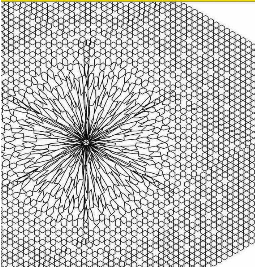
Figure 4, The Chirality principle and structure of the oscillating Dark Energy Higgs vacuum lattice.
