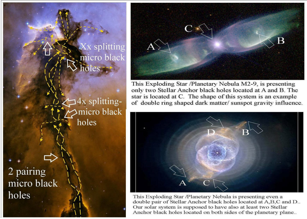
Figure: 11. examples of dual pairs of stellar anchor black holes and the so called Spire creation of star forming dust pillars by a splitting and pairing black hole, also proposed for the fast galaxy formation after the big bang. ( fig 12)
