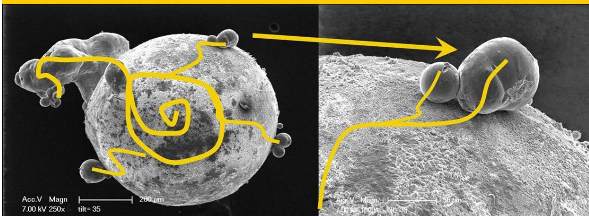
Figure 20. Comparison between LHC (CERN) UFO dust particles (10 \mu\text{m} ) with molten Silicon globules (100 \mu\text{m} ) originated in the lab by travelling and evaporating Interference Quantum Knots (micro dark Matter Black Holes)
