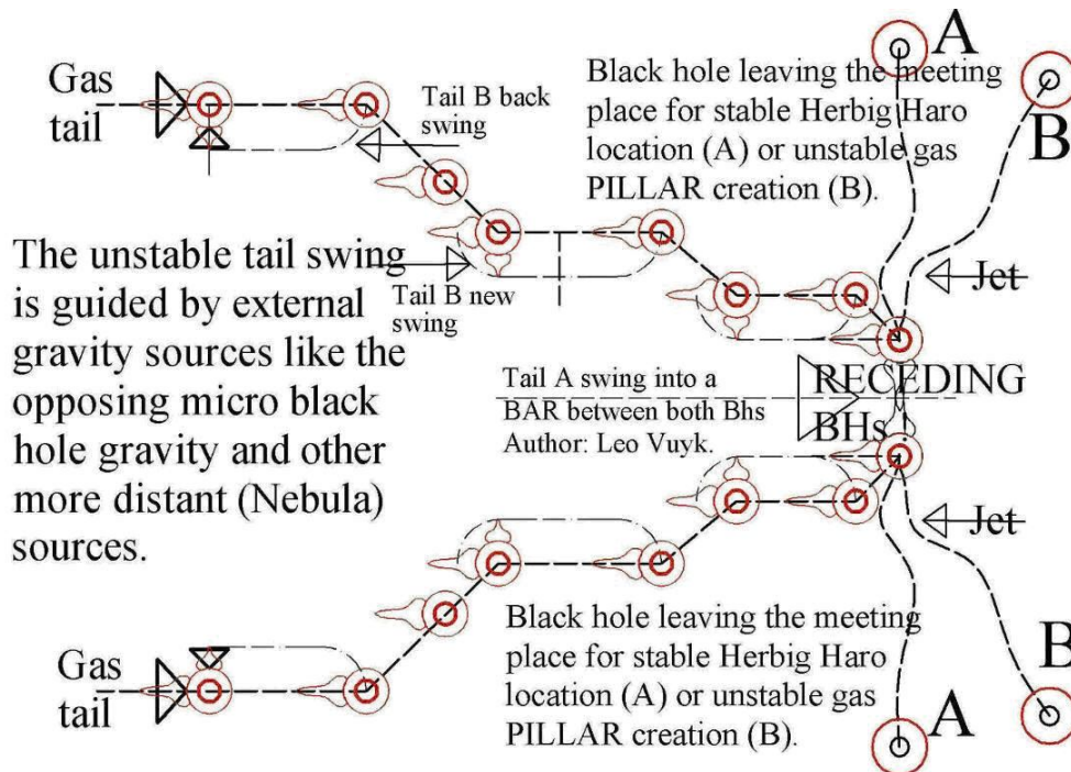
Figure 8, New Black hole propulsion principle by a self produced plasma-dust tail,. As a consequence, New black holes do not merge to form larger nuclei, they even repel negative charged metal surfaces by their own exterior electron charge. ( see also fig. 9)
