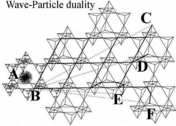
Photon trajectories through the tetrahedral Chiral vacuum lattice.
