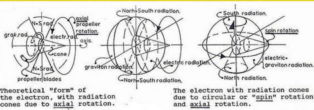
Figure 14, The polarisation of the double spinning propeller shape of Fermions is the origin of the monopole radiation differences radiated into different directions from the Fermion radiation area around the centre. It is assumed that electric and gravity radiation is not mixing with magnetic monopole radiation inside the magnetic double cone area. Consequently, the measured difference between the Equatorial gravity (9.78 m/sec 2 ) and Polar gravity (9.83 m/sec 2 ) should be greater without this effect.
