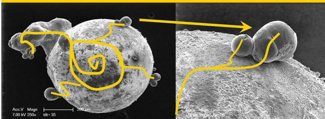
Figure 21. An other example of Quantum Knot heated globules found on an exploded battery. Suggestion for the origin of external stainless steel globules found on the Boeing 787 Dreamliner APU battery damage jan.7.2013 at Boston airport. Discharge Quantum Knot black holes seem to be able to melt stainless steel! Melting point of stainless steel is 3000 degree C! ( Globule diameter 30-120 mu.meter)
