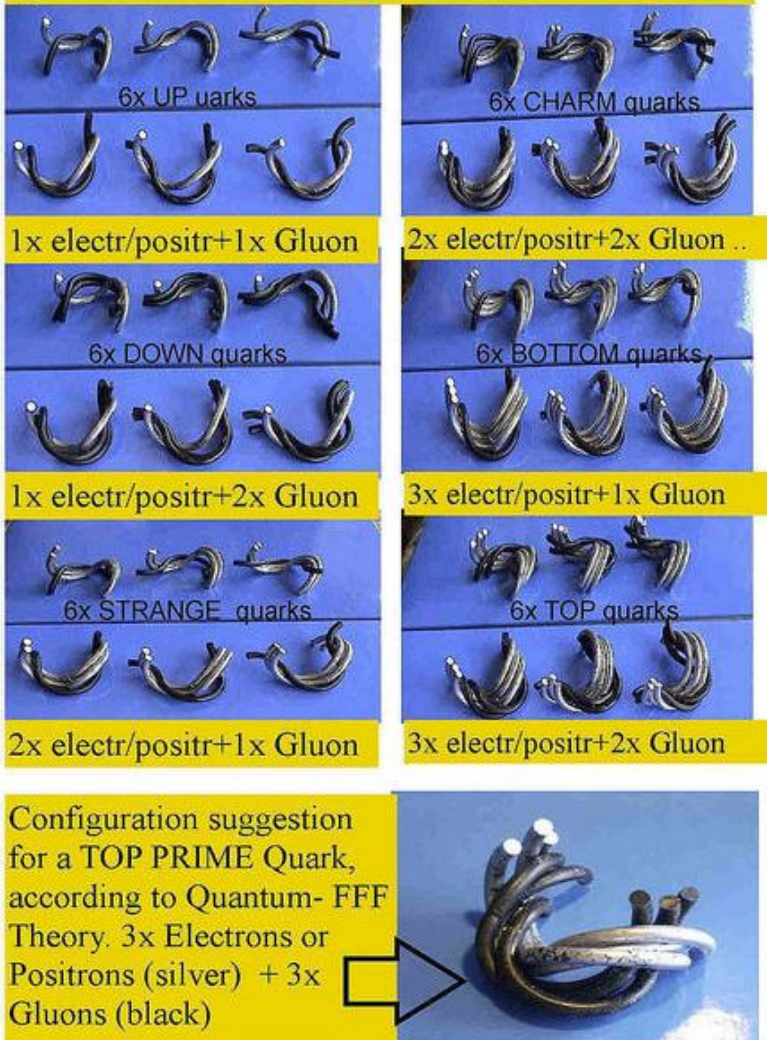
Figure 17, 5x different shaped Photon/Gluons can combine with the two propeller shapes of the Electron and Positron to form all coloured (QCD) Quarks and even a so called Top Prime Quark. The Muon and Tau particle are supposed to be the same as the Down quark, respectively the Charm quark.
