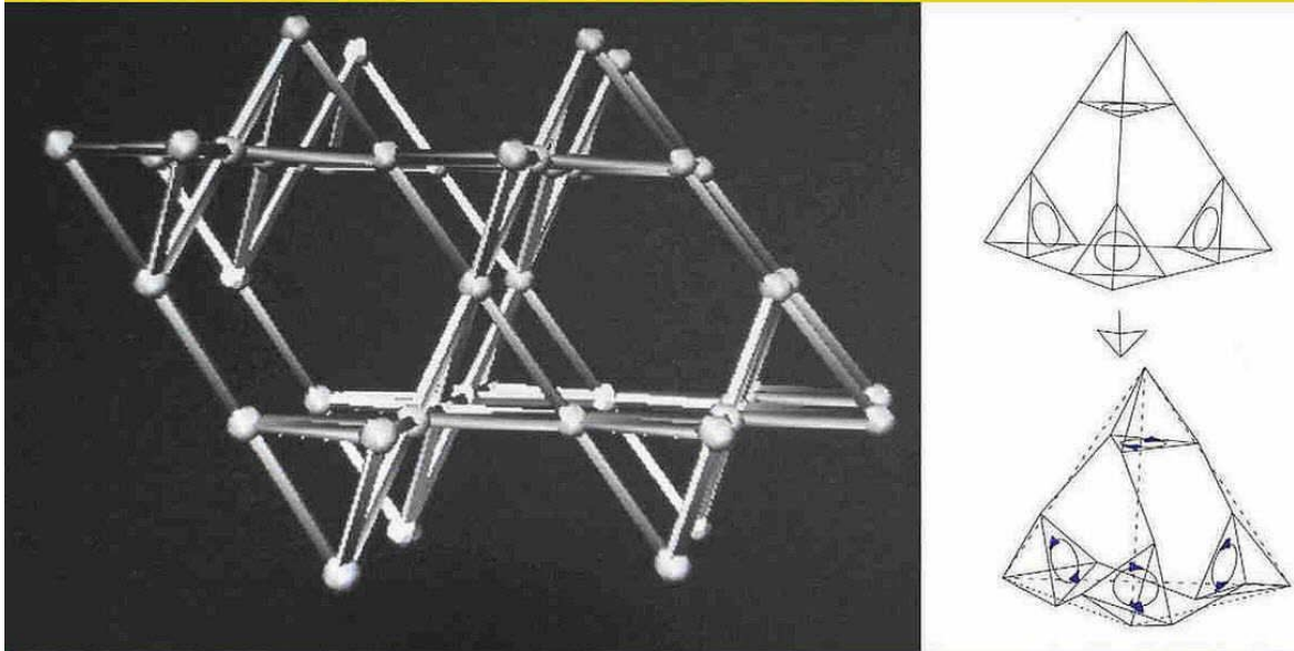
Symplified tetrahedral vacuum lattice structure (left), constructed by complex chiral tetrahedral building blocks (right). Each universe has to choose between a left- or righthanded rotation of its tetrahedral building blocks. Each chiral lattice has the Planck length and is supposed to be equipped with at least two oscillating massless new Higgs particles.
