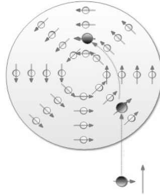
Figure 5.3: Proton in "magnetic" field
