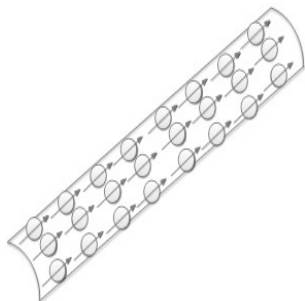
Figure 5.1: Organized electron spinning vectors
