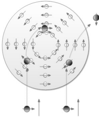
Figure 5.4: Electron in “magnetic” field
