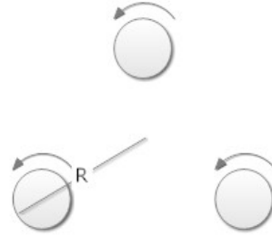
Figure 6.1: Proton
