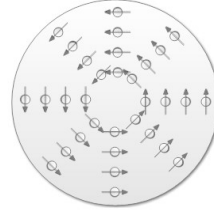
Figure 5.2: Magnetic pole from above
