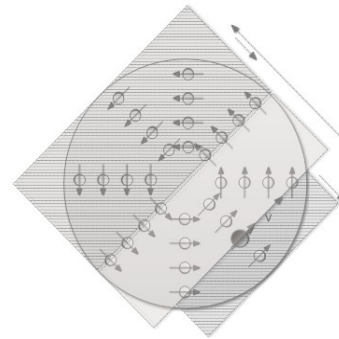
Figure 5.5: Effective interaction area
