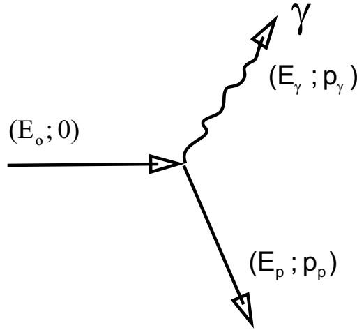
Figure 21: Feynman diagram
