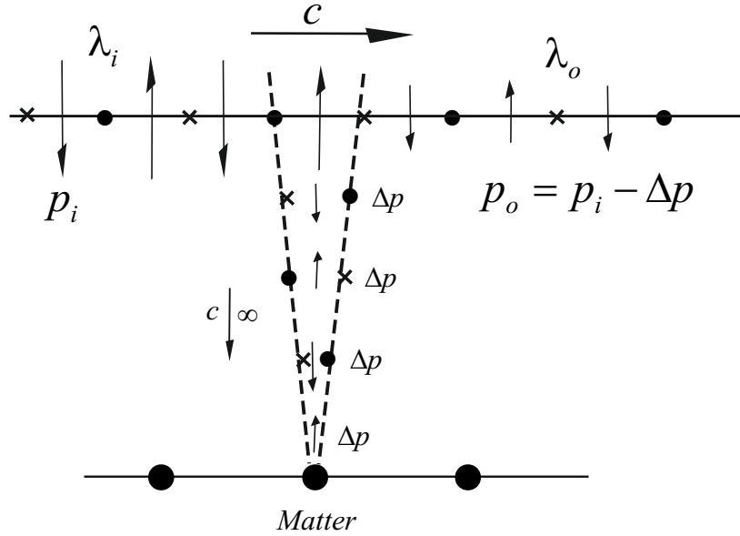
Figure 26: Loss of energy of a BSP with v = c
