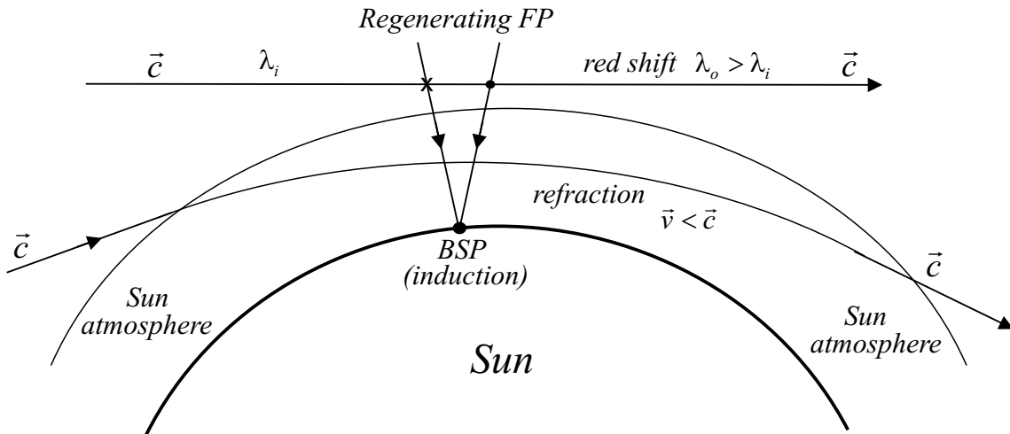
Figure 27: Refraction and red-shift at the Sun
