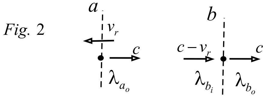
Figure 24: Sagnac experiment
