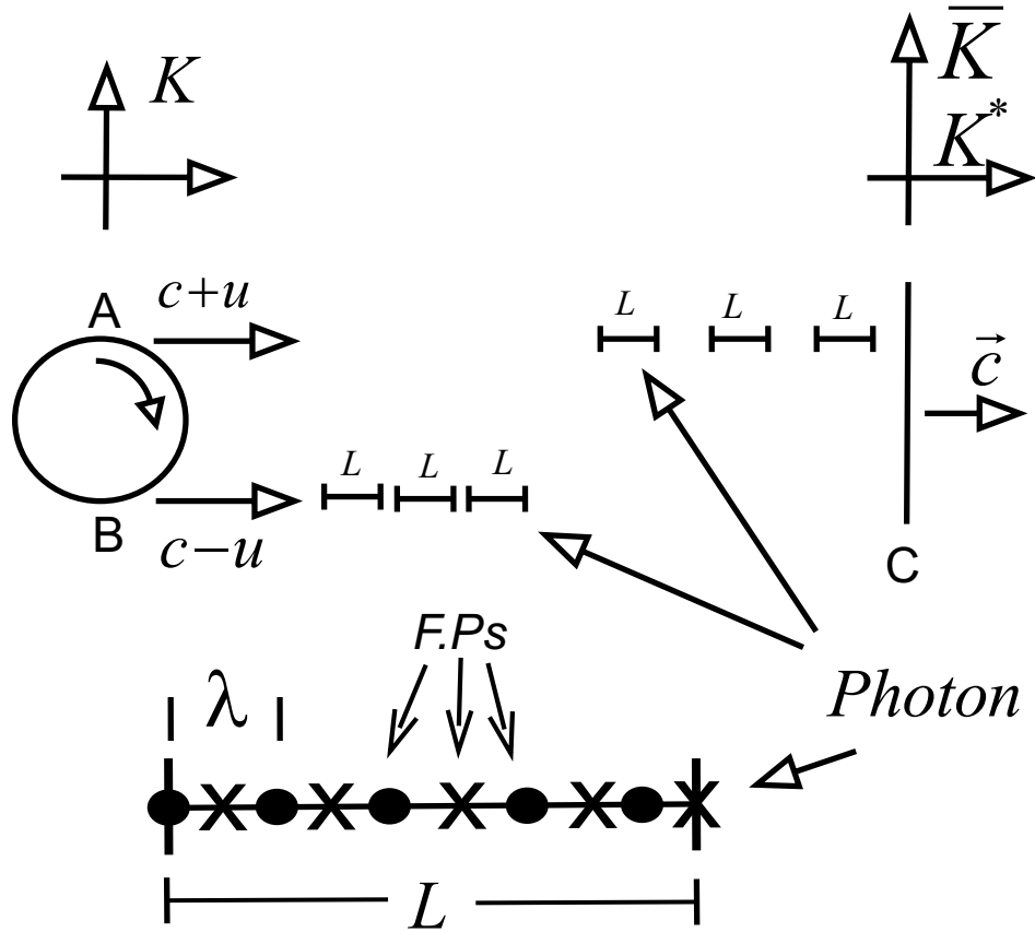
Figure 22: Emission Theory.
