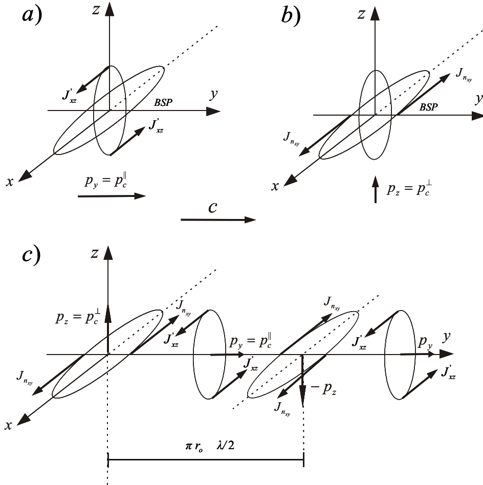
Figure 25: Different forms of BSP with light speed
