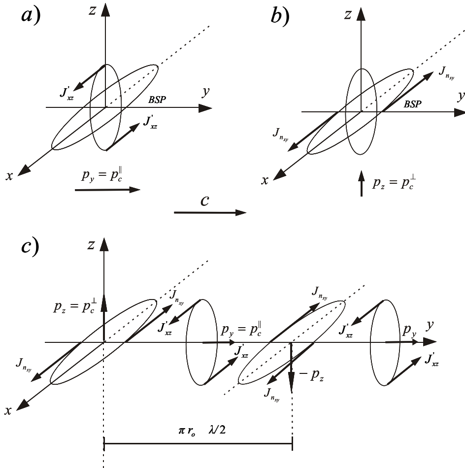
Figure 33: Different forms of BSP with light speed
