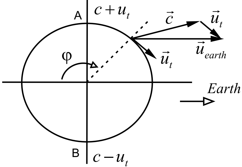
Figure 30: Speed of photons at an Binary Pulsar.
