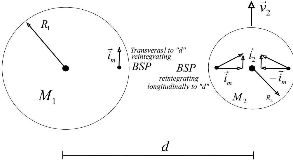
Figure 16: Ampere gravitation
