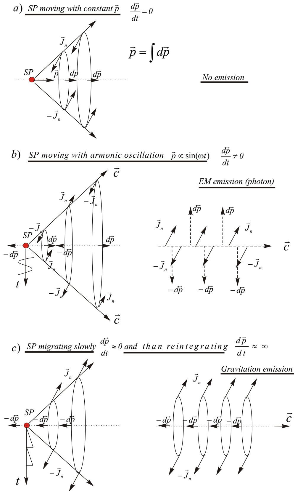
Figure 21: Electromagnetic and Gravitation emissions
