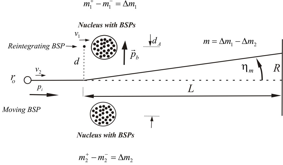
Figure 12: Bending of BSPs
