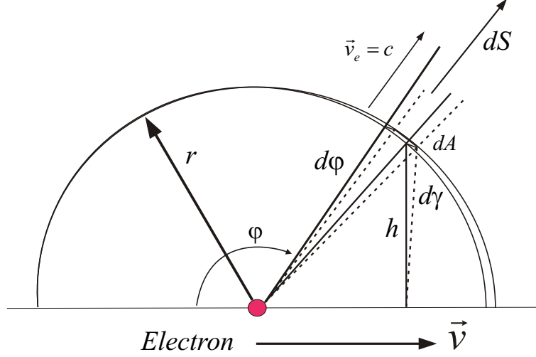
Figure 19: Emitted Energy flux density dS of a moving electron
