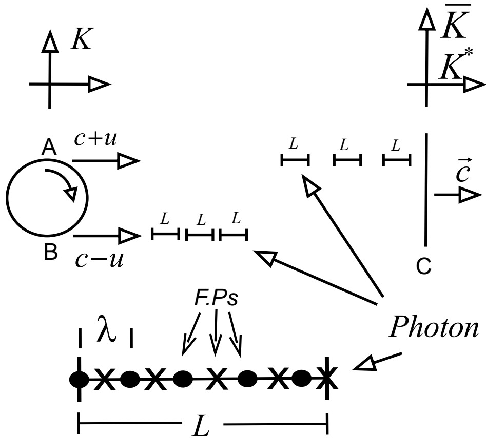
Figure 27: Emission Theory.
