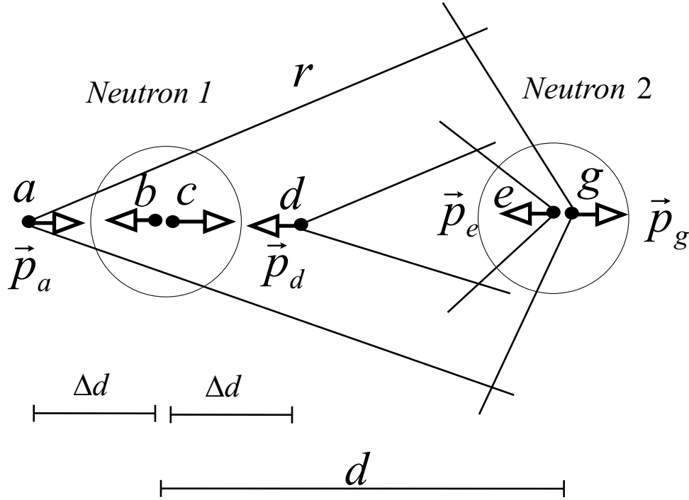
Figure 14: Net momentum transmitted from neutron 1 to neutron 2
