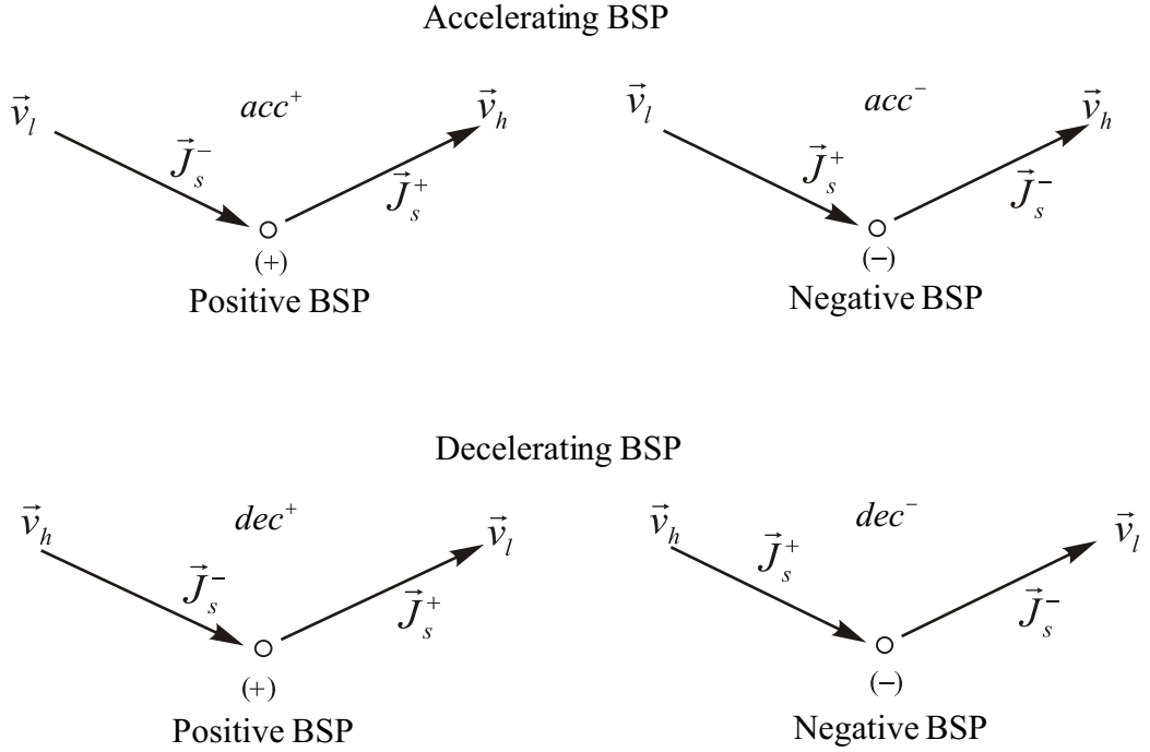
Figure 22: Conventions for BSPs
