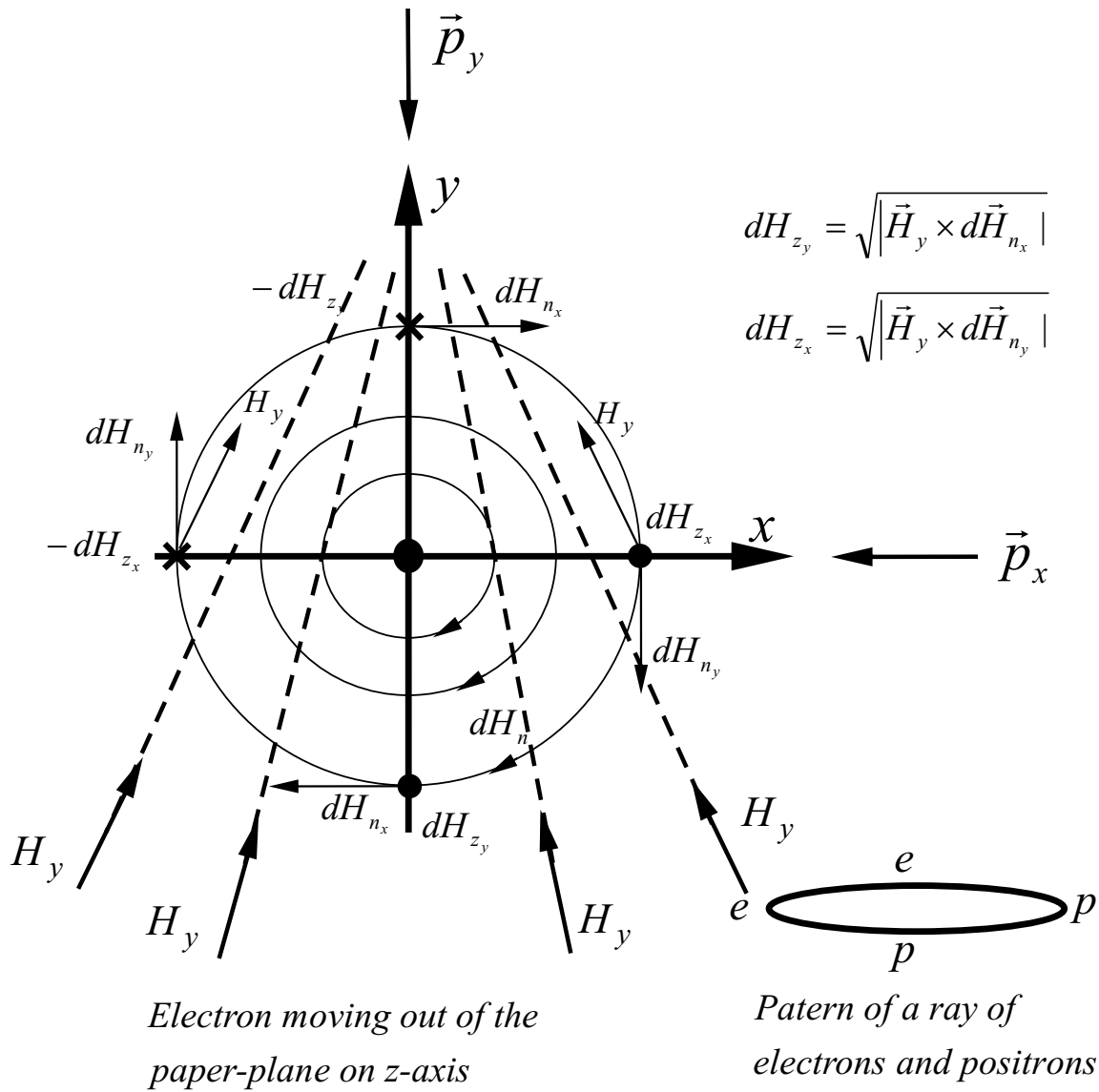
Figure 11: Stern-Gerlach-experiment with an inhomogeneous magnetic field
