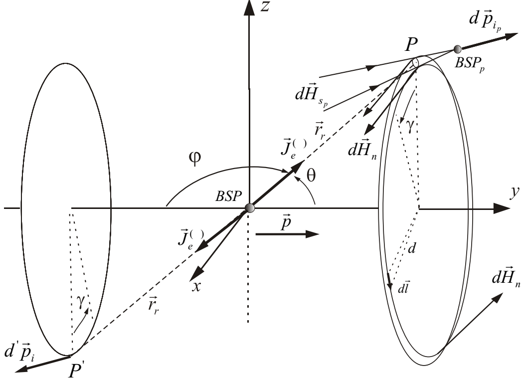
Figure 13: Linear momentum balance between static and moving BSPs
