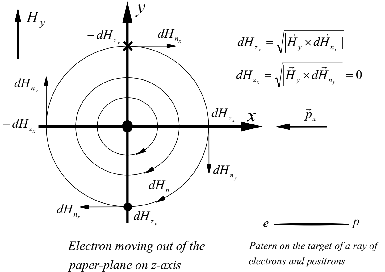
Figure 10: Stern-Gerlach-experiment with an homogeneous magnetic field
