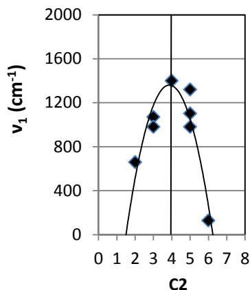
Fig. 6. A graphic produced as a cross-check while data were being introduced into the portion of the main file for molecules with n_e = 21 . Vibration frequencies v_1 are plotted on C_2 . C_2 = 0 and 8 relate to rare-gas molecules. The parabolic fit has only a suggestive role; a more realistic curve might intersect the abscissa at 1 and 7. The very low-value datum at C_2 = 6 would normally have been ignored but in this case was retained. The figure gives a sense of the spreads of data for which averages and error measures were calculated. Additional discussion of these measures follows in Section 4.3.
