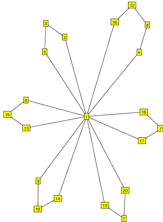
FIGURE 37. G_{20}^3 \cong C_5 \times C_4 , subgroup of S_5 . (4^5, 5^1) .
