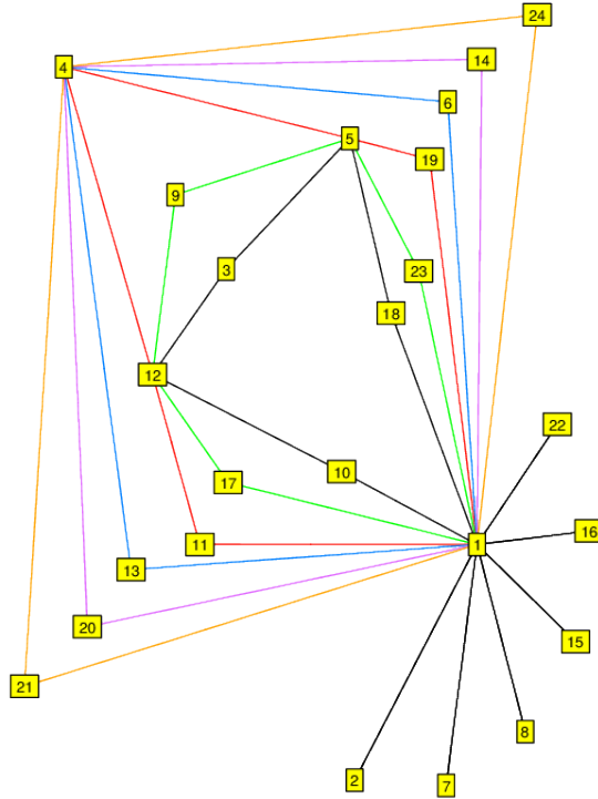
FIGURE 48. G_{24}^8 \cong (C_6 \times C_2) \times C_2 , subgroup of S_7 . (2^6, 4^3, 6^3) .
