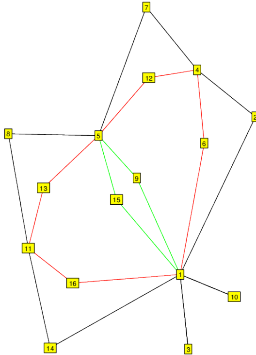
FIGURE 22. G_{16}^5 \cong C_8 \times C_2 . (2^2, 4^1, 8^2) .
