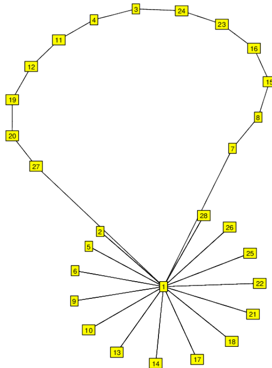
FIGURE 63. G_{28}^3 \cong D_{28}. (2^{14}, 14^1) .
