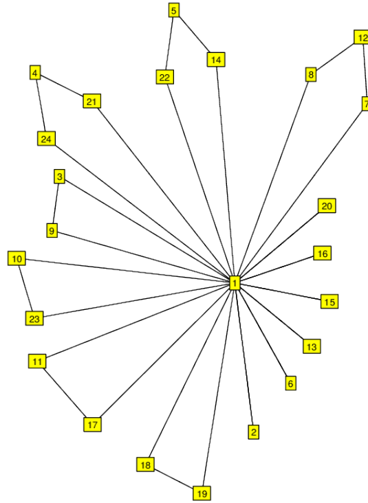
FIGURE 52. G_{24}^{12} \cong S_4. (2^6, 3^4, 4^3) .
