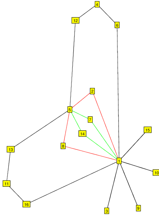
FIGURE 25. G_{16}^8 \cong QD_{16} , subgroup of S_8 . (2^4, 4^2, 8^1) .
