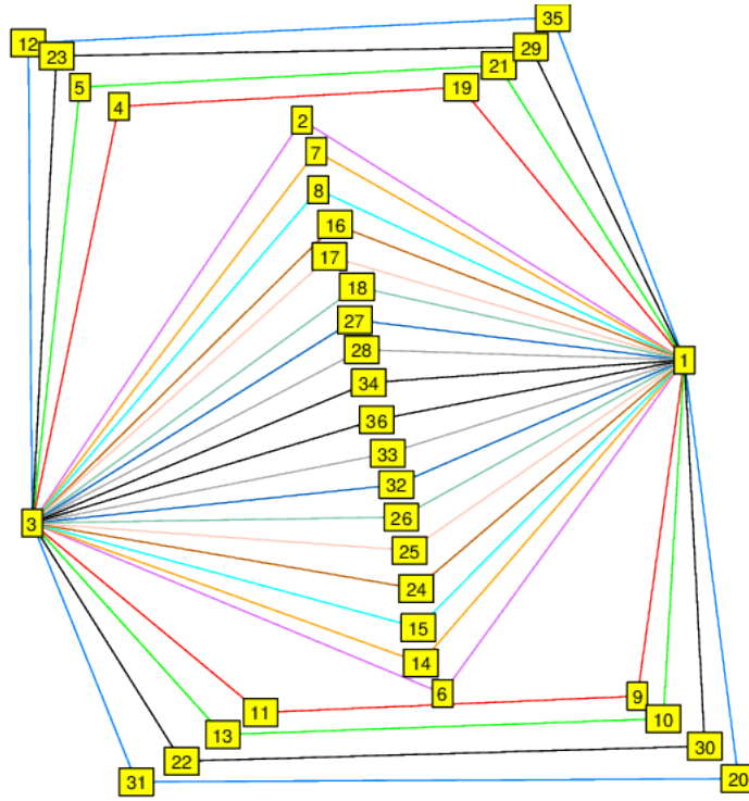
FIGURE 124. G_{36}^7 \cong (C_3 \times C_3) \rtimes C_4 . (4^9, 6^4) .
