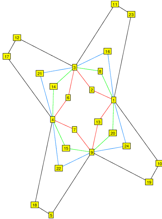
FIGURE 42. G_{24}^1 \cong C_3 \times C_8 . (8^3, 12^1) .
