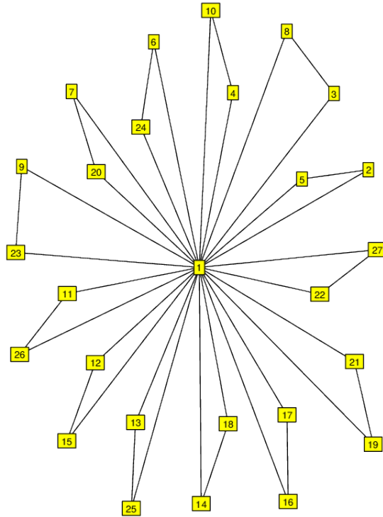
FIGURE 59. G_{27}^3 \cong (C_3 \times C_3) \times C_3 . ( 3^{13} ).
