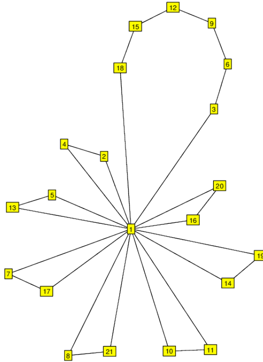
FIGURE 40. G_{21}^1 \cong C_7 \times C_3 , subgroup of S_7 . (3^7, 7^1) .
