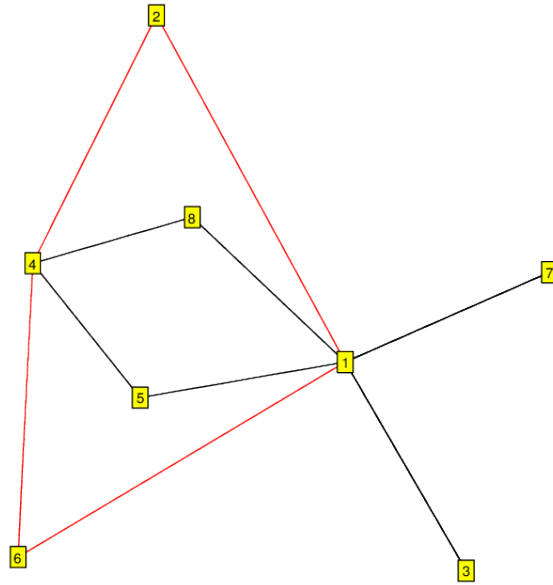
FIGURE 8. G_8^2 \cong C_4 \times C_2 , subgroup of S_6 . (2^2, 4^2) .
