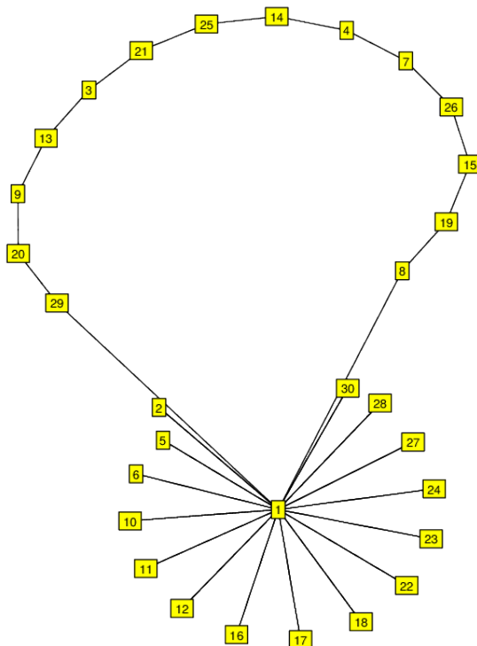
FIGURE 67. G_{30}^3 \cong D_{30}. (2^{15}, 15^1).
