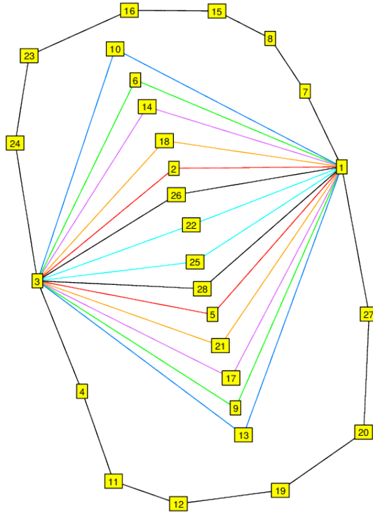
FIGURE 62. G_{28}^1 \cong C_7 \times C_4. (4^7, 14^1) .
