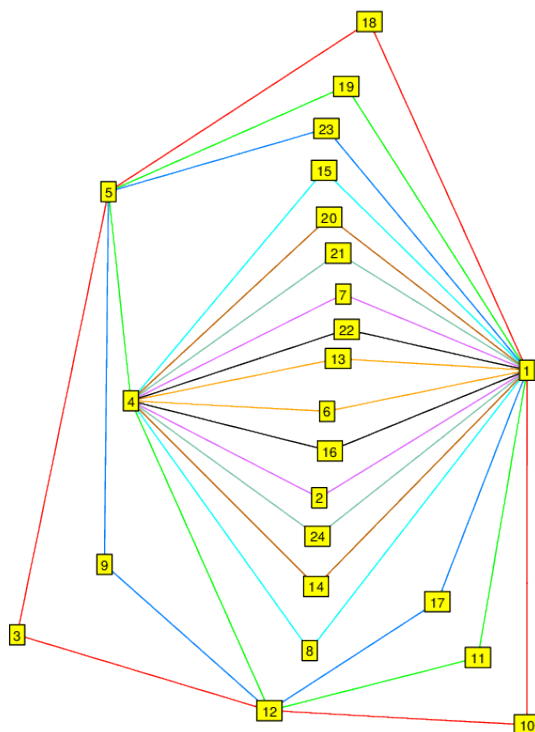
FIGURE 47. G_{24}^7 \cong C_2 \times (C_3 \times C_4) , subgroup of S_9 . (4^6, 6^3) .
