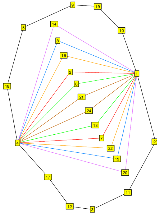
FIGURE 44. G_{24}^4 \cong C_3 \times Q_8 . (4^6, 12^1) .
