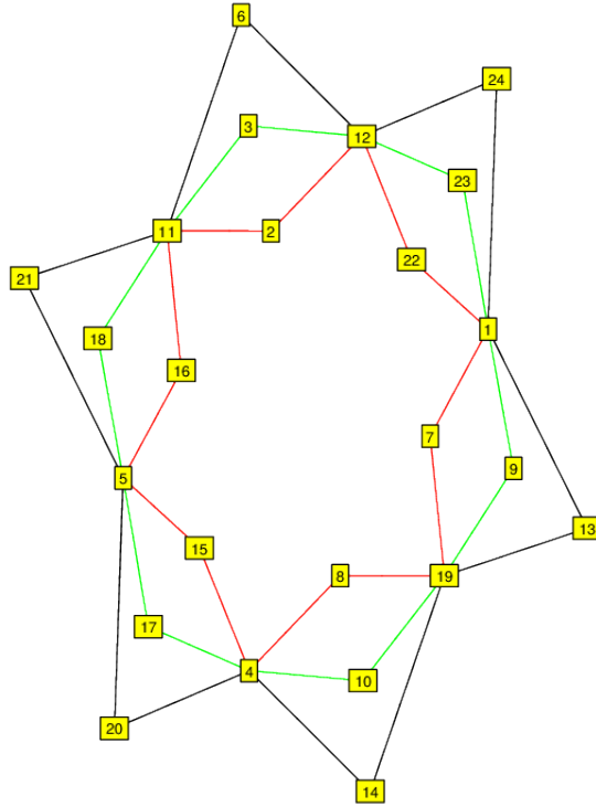
FIGURE 51. G_{24}^{11} \cong C_3 \times Q_8 . (12^3) .
