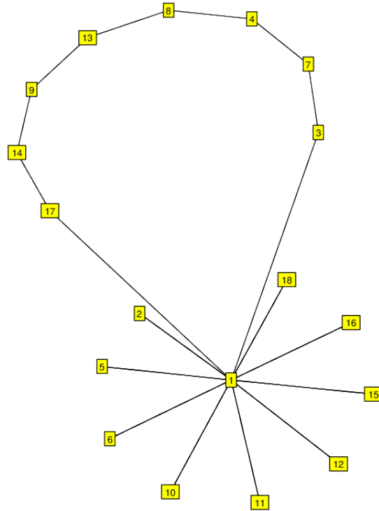
FIGURE 32. G_{18}^1 \cong D_{18} , subgroup of S_9 . (2^9, 9^1) .
