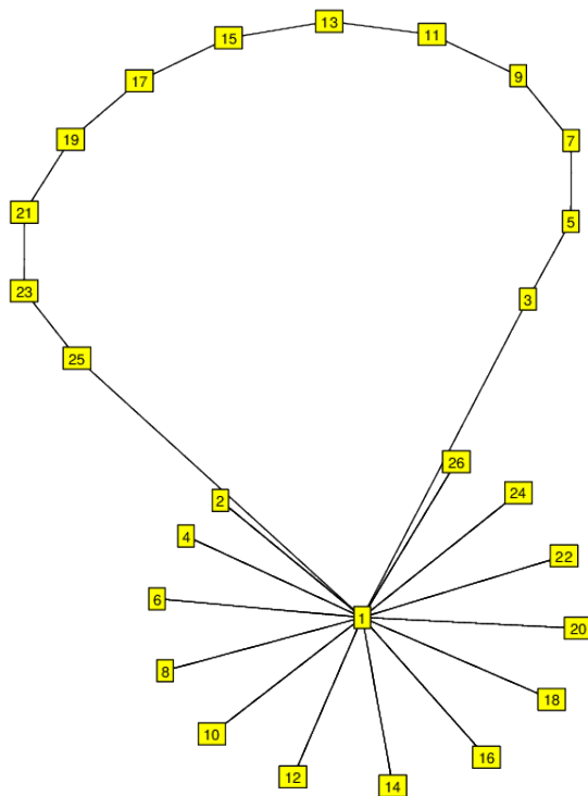
FIGURE 57. G_{26}^1 \cong D_{26}. (2^{13}, 13^1).
