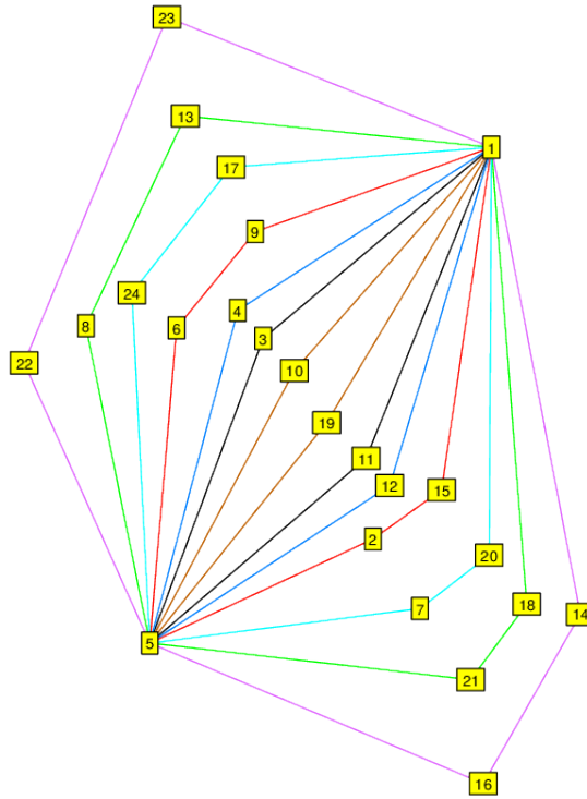
FIGURE 43. G_{24}^3 \cong SL(2, 3) , subgroup of S_8 . (4^3, 6^4) .
