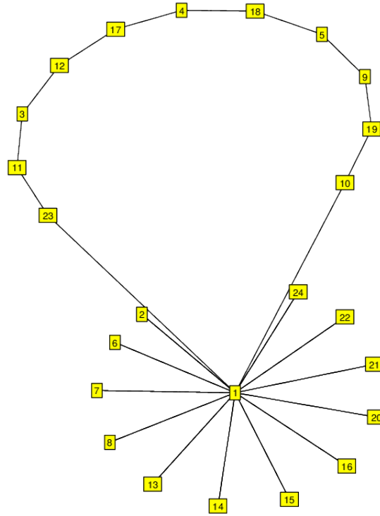
FIGURE 46. G_{24}^6 \cong D_{24} , subgroup of S_7 . (2^{12}, 12^1) .
