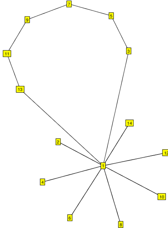
FIGURE 18. G_{14}^1 \cong D_{14} , subgroup of S_7 . (2^7, 7^1) .
