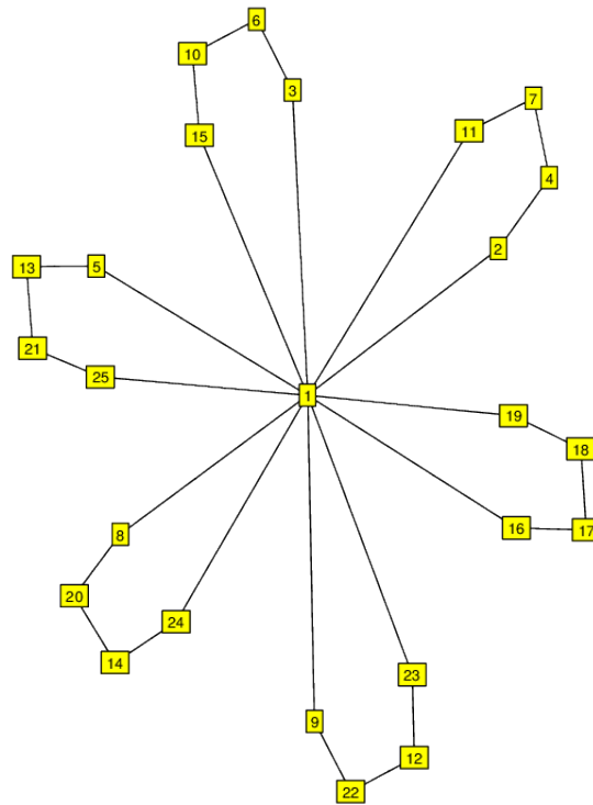
FIGURE 56. G_{25}^2 \cong C_5 \times C_5 . (5 6 ).
