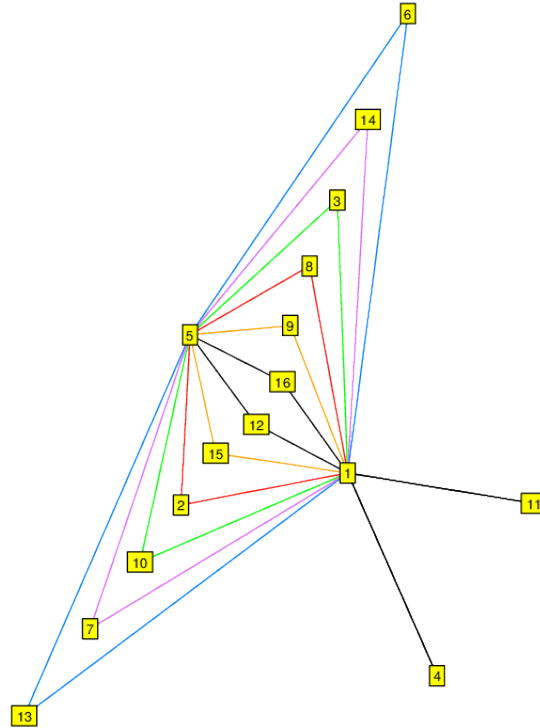
FIGURE 29. G_{16}^{12} \cong C_2 \times Q_8, (2^2, 4^6) .
