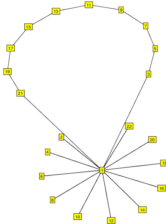
FIGURE 41. G_{22}^1 \cong D_{22} . (2^{11}, 11^1) .
