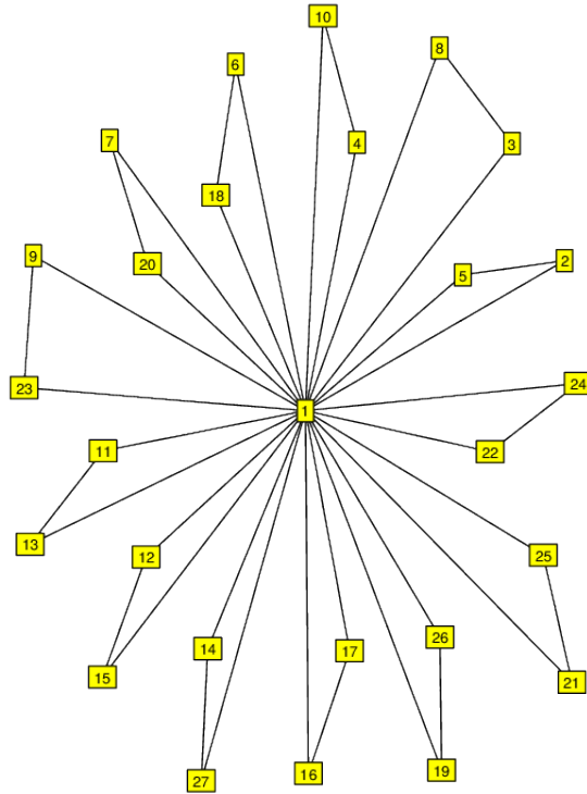
FIGURE 61. G_{27}^5 \cong C_3 \times C_3 \times C_3 . ( 3^{13} ).
