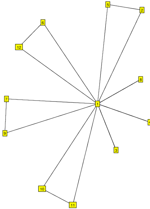
FIGURE 15. G_{12}^3 \cong A_4 , subgroup of S_4 . (2^3, 3^4) .
