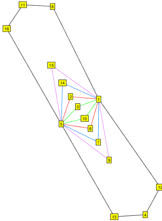
FIGURE 26. G_{16}^9 \cong Q_{16} \cdot (4^4, 8^1) .
