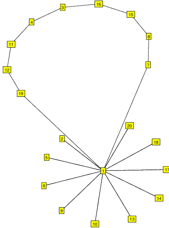
FIGURE 38. G_{20}^4 \cong D_{20} , subgroup of S_7 . (2^{10}, 10^1) .
