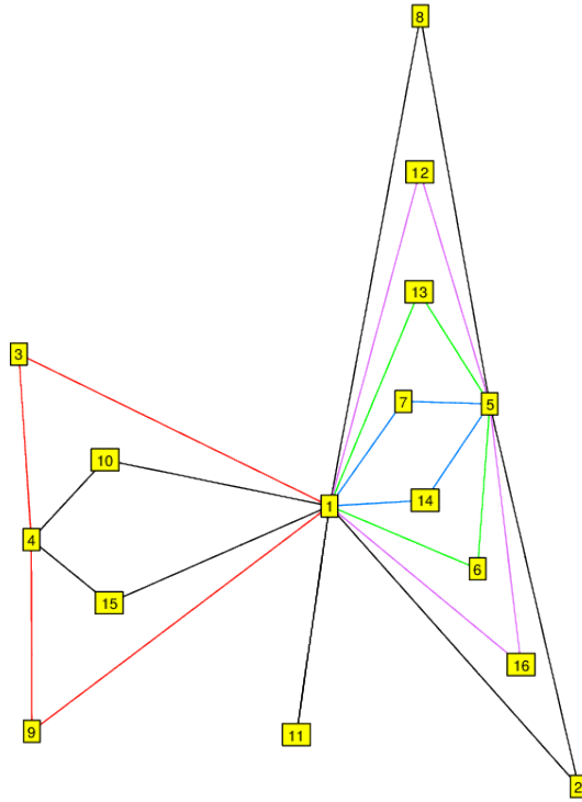
FIGURE 21. G_{16}^4 \cong C_4 \times C_4 , subgroup of S_8 . (2^1, 4^6) .
