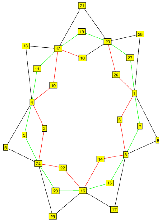
FIGURE 64. G_{28}^4 \cong C_{14} \times C_2 . (14^3) .
