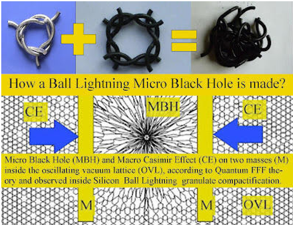
Figure 12. Quantum Knots as dark matter black holes eating the vacuum and the origin of so called Casimir gravity on black holes.
