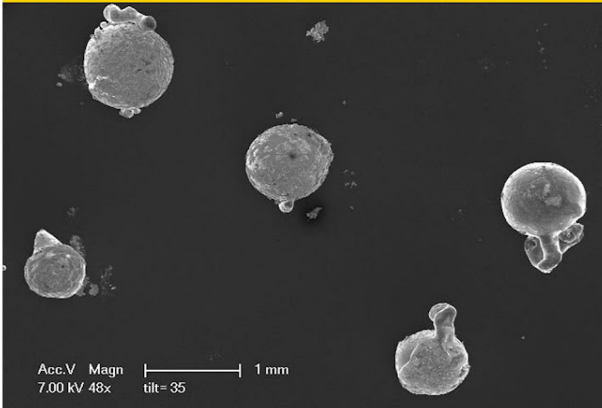
Figure 1 , Image of some silicon nuclei, all with globular shape and equipped with one large and several smaller appendices and diameters between 0.4 and 0.8 mm
