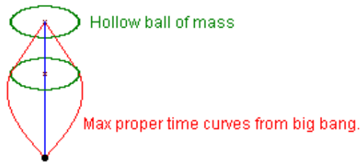
Fig. 1. The gradient of the scalar field of time is along the blue curve that is the Schwarzschild time coordinate but slightly displaced from the center, the gradient is along the red curves which result in discontinuity unless non-geodesic curvature is involved, i.e. non-inertial acceleration.
