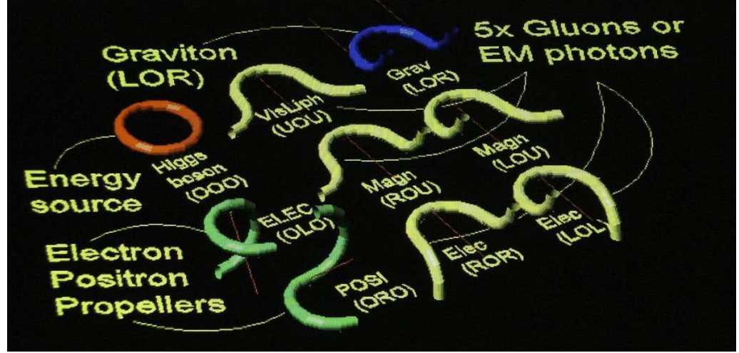
Figure 10, The particle zoo of single ELEMENTARY particles made out of ONE convertible Torus shaped Higgs particle, equipped with three hinges of 90 degree rotation.
