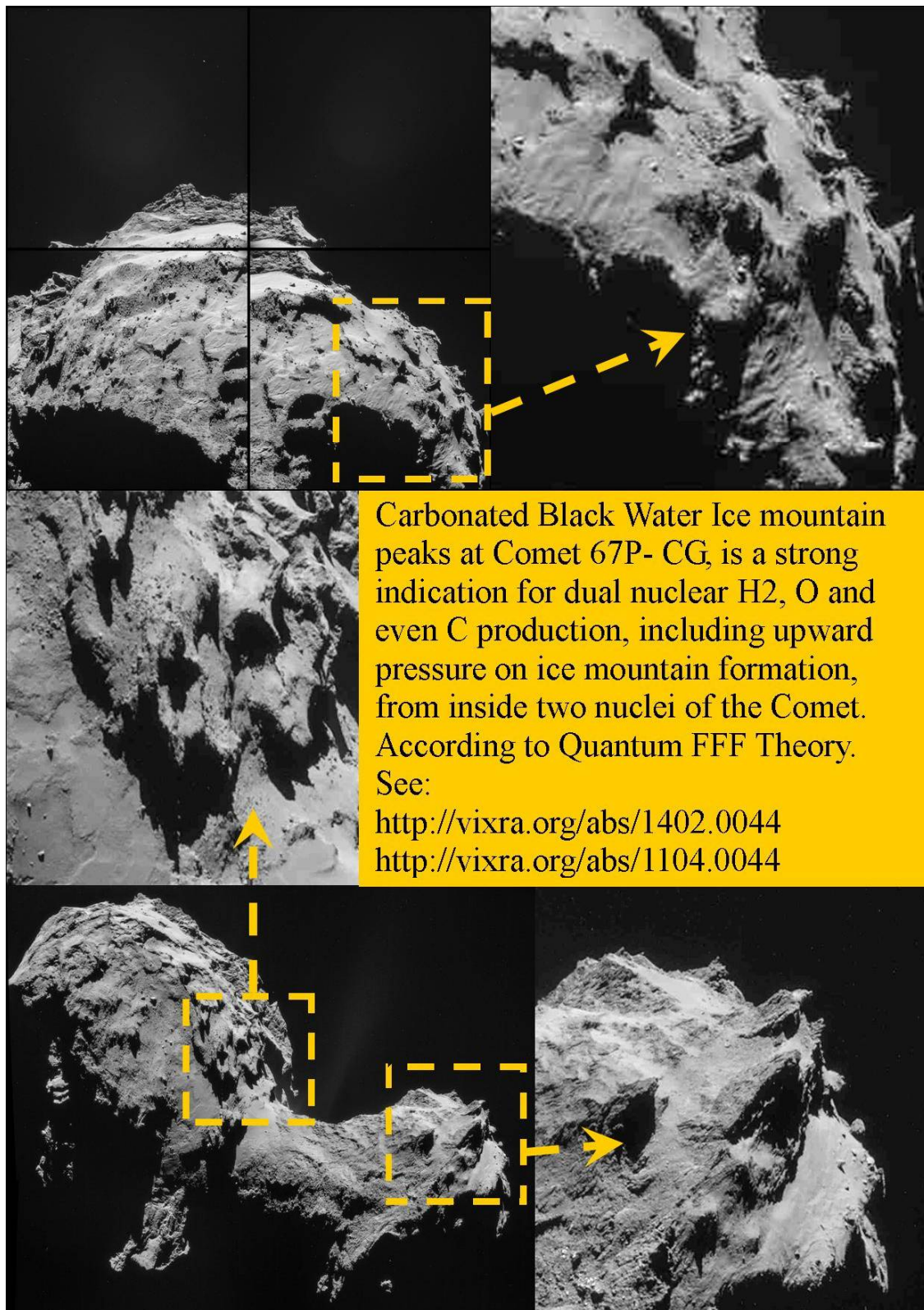
Figure 20, NOT EROSION but Plate tectonics driven by the nuclear matter production of new paradigm dark matter black holes.
