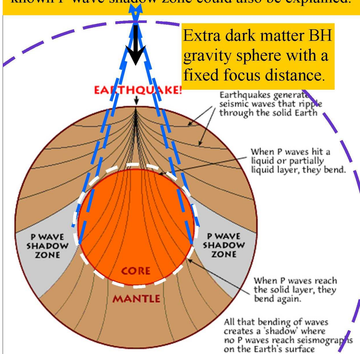
Figure 25, According to Quantum FFF Theory, (Function Follows Form) Microscopic Electric Dark Matter Black Holes are proliferated inside stars (sunspots), Comets and ball lightning. Now the TGD model (27-dec. 2014, Matti Pitkanen) suggested that a dark matter sphere around earth, could solve the Flyby anomaly. If the sphere is located inside earth however the well known P wave shadow zone inside the earth, could also be explained.
