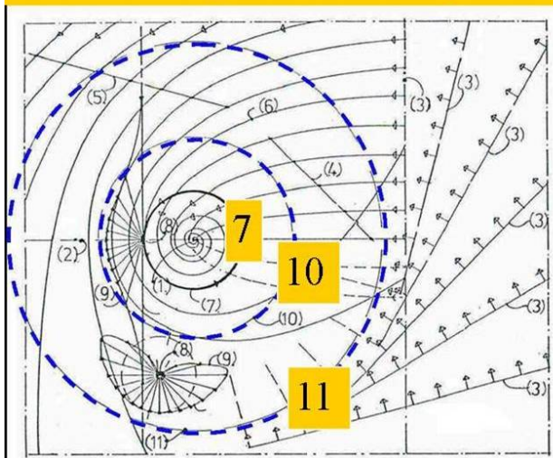
Figure: 15. Fermion repulsion principle around dark matter black holes producing water ice Comets Megacryometeors. A special example of nuclear water ice production is found in the Moon Hyperion, which is assumed to be a former Comet, left alone by its Black Hole energy source.
