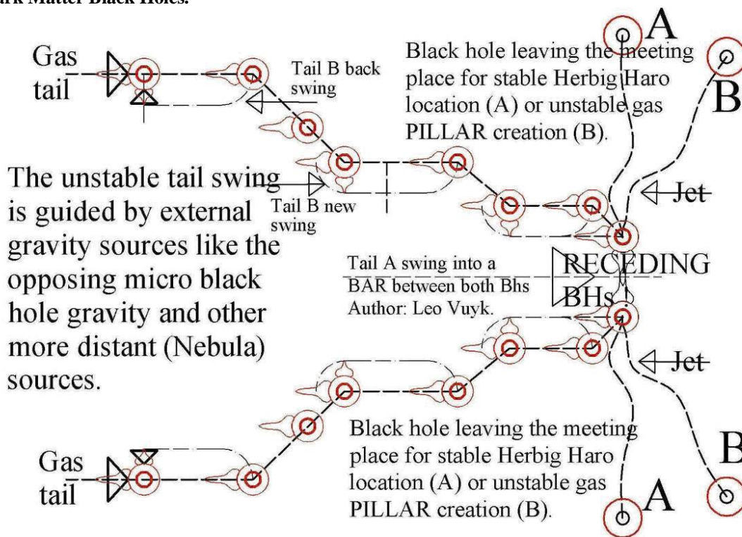
Figure 6, New Black hole propulsion principle by a self produced plasma-dust tail,. As a consequence, New black holes do not merge to form larger nuclei, they even repel negative charged metal surfaces by their own exterior electron charge. ( see also fig. 9)
