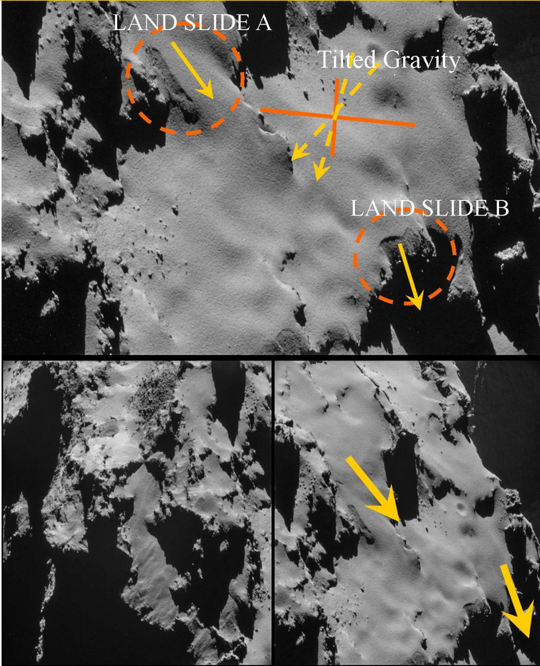
Figure 24, Anomalous non perpendicular surface Gravity problem.
