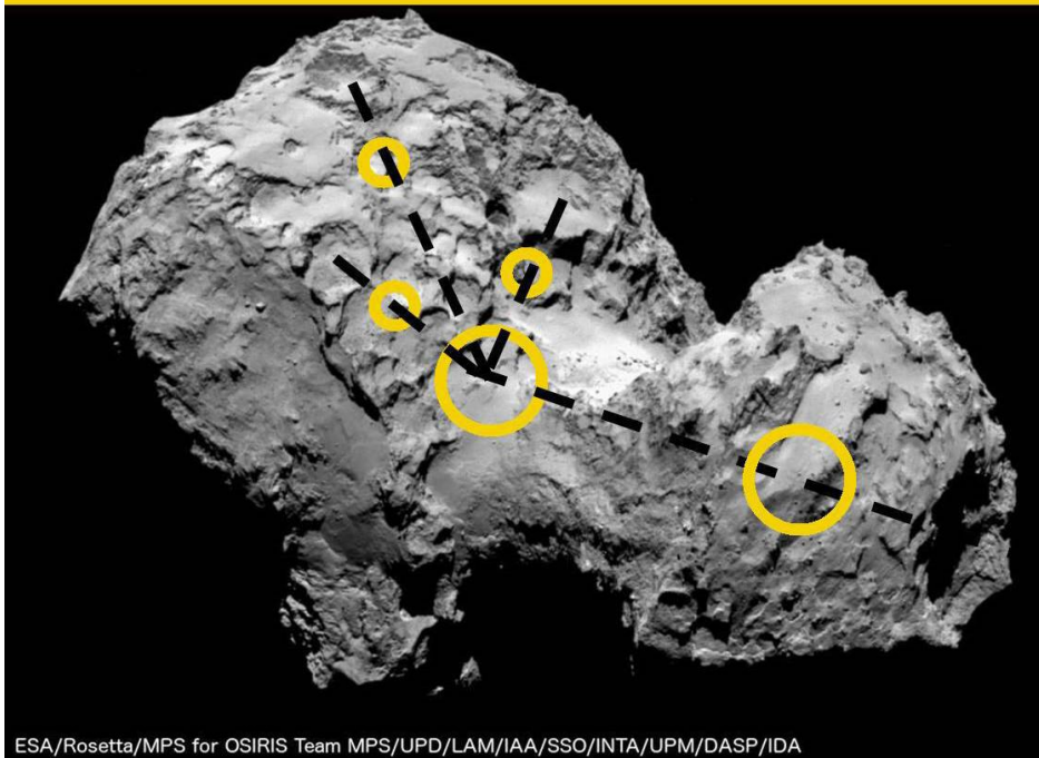
Figure: 16, Proposal for the origin of circular craters at Comet 67p C-G.
