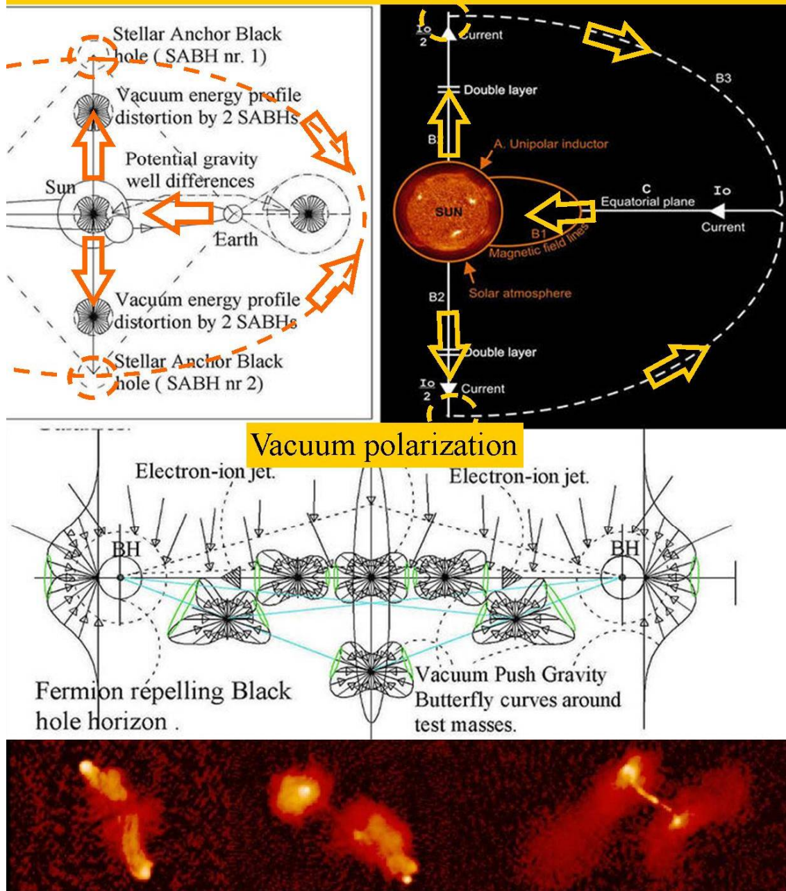
Figure: 8. Black hole propulsion and pairing principle of fig 8, seems to be the origin of dual Stellar or galaxy Anchor black holes (see figure 11) and even so called Birkeland /Alfven current circuits around stars and galaxies by vacuum polarization. The energetic polarized vacuum oscillation spectrum is the motor for fast gas and electron transport starting direct after the big bang.
