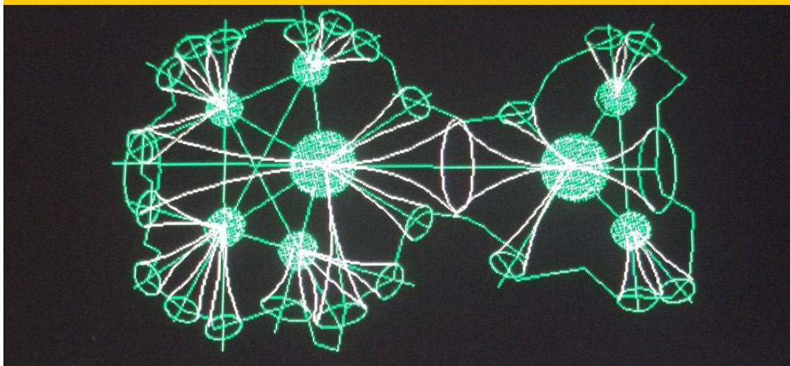
Figure 26, Internal Porous Funnel Structures, created by Dark Matter BH point sources for Comet 67PCG, and Hyperion. (A former Comet left alone by its former Dark Matter BH nucleus).
