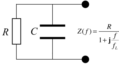
Figure 3. Resistor shunted by a capacitor.
