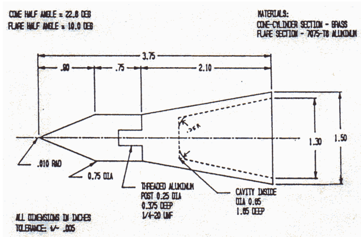
Figure-1. Sketch of Cone-Cylinder-Flare Body
