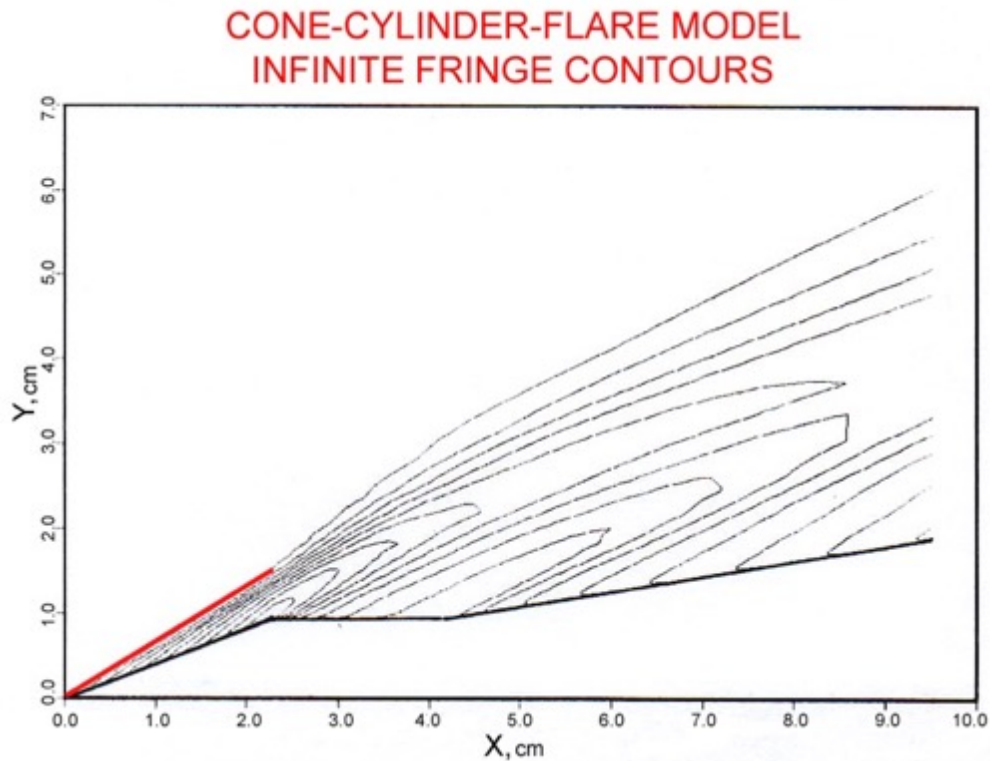
Figure-4, Theoretical Interferogram
