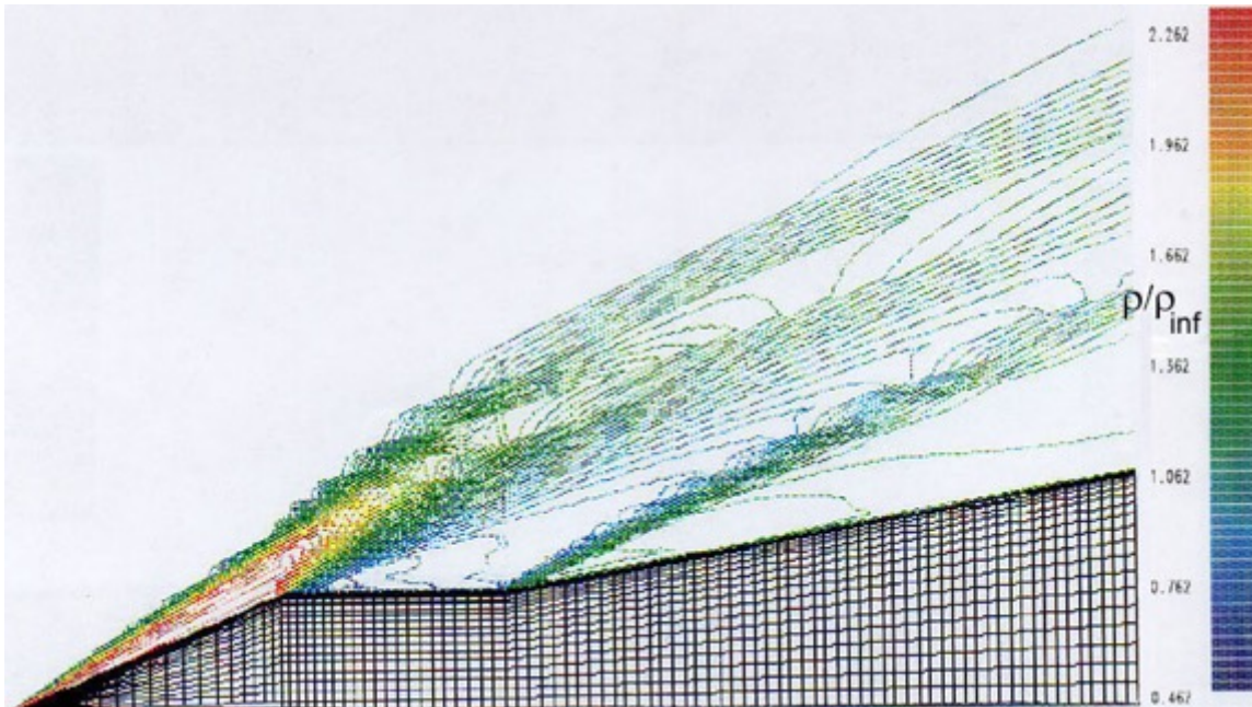
Figure-5, EAGLE Density Contours
