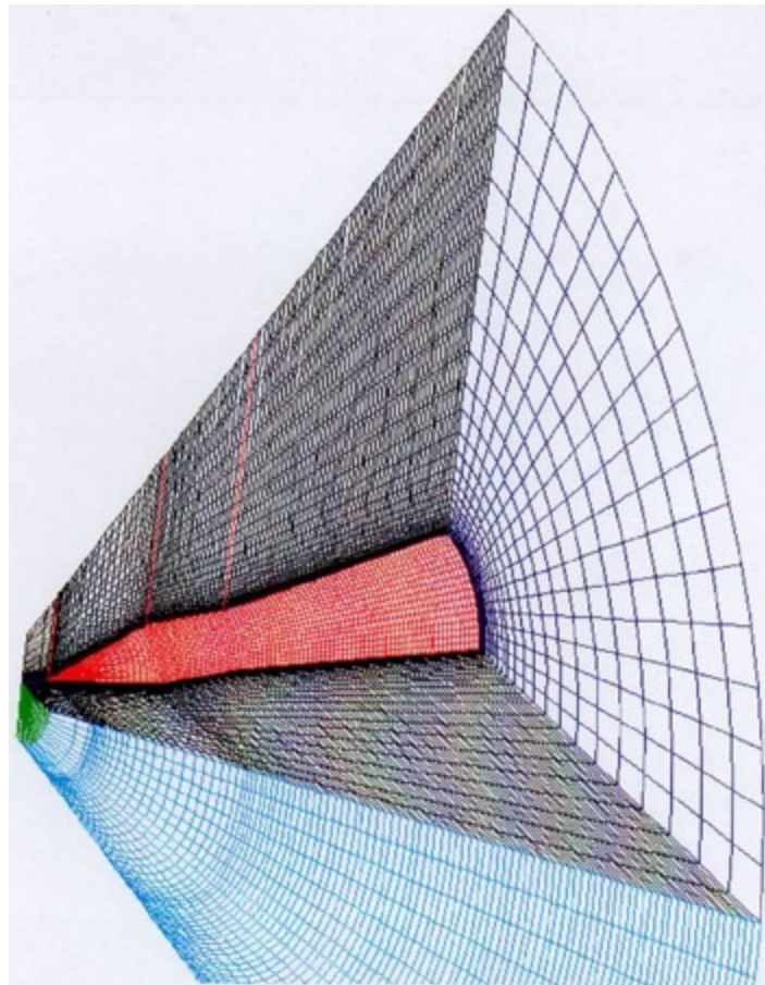
Figure-3, Four Block EAGLE Grid
