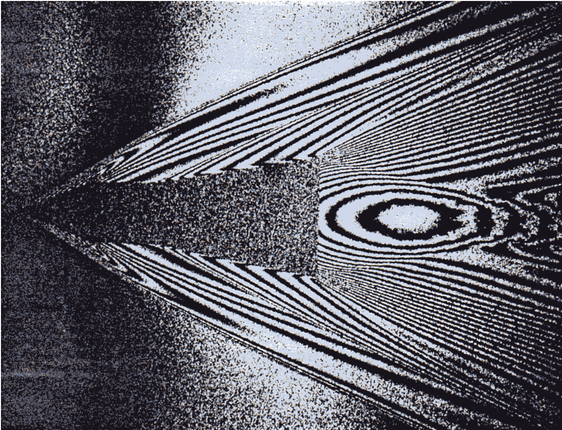
Figure-2 Experimental Interferogram
