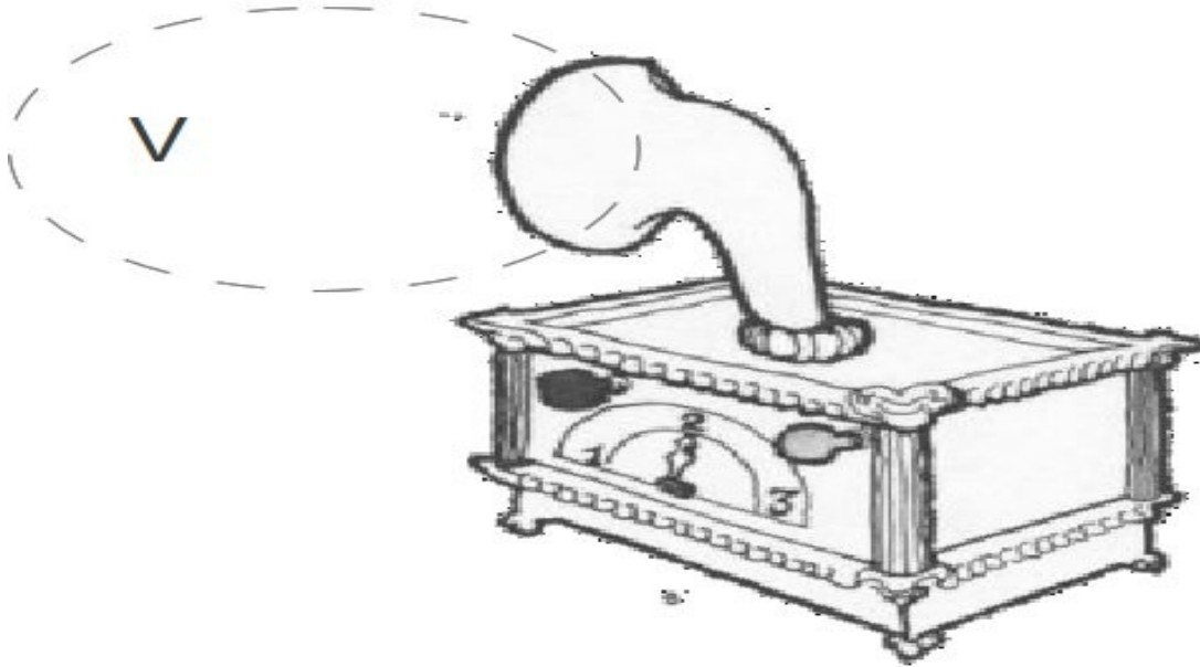
Figure 1. A detector is pictured as sampling particle flux from a volume V at a time t . The reading on the detector is the output of a probabilistic mapping of variables \lambda internal to the volume V . Adapted from [Mermin, 1985].
