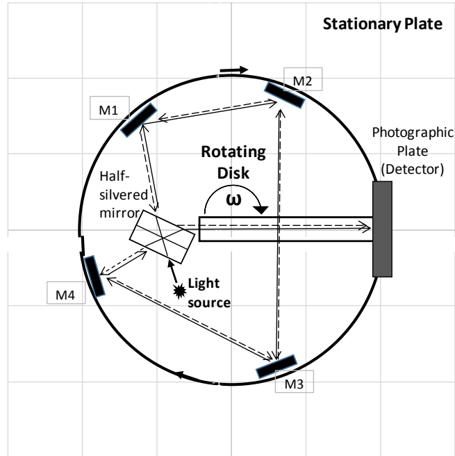
Fig.3 Schematic representation of the Sagnac interferometer
