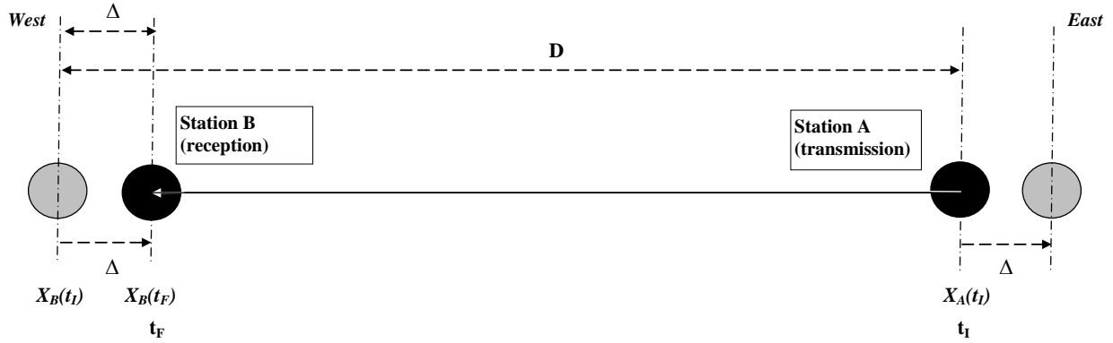
Fig.2. One-way light speed determination – westward transmission
