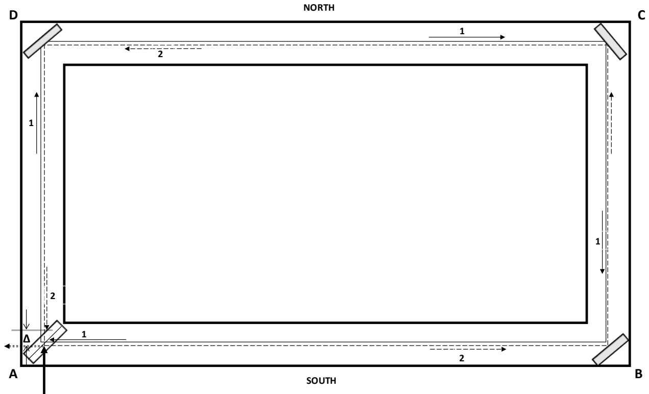
Figure 6. The scheme of the Michelson-Gale-Pearson experiment
