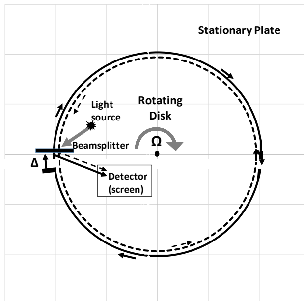
Fig.4 Schematic representation of a fiber optic interferometer
