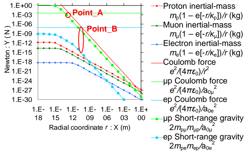
FIG. 3. The scalable inertial mass of fermions, and the Coulomb force and the elementary gravity of a combination thereof. The red / green / blue dotted lines are the scalable inertial mass curves of each fermion. The solid lines are the line that Coulomb force. The Yellow-green / light-blue dotted lines (proton-muon, proton-electron) are the elementary gravity line.
