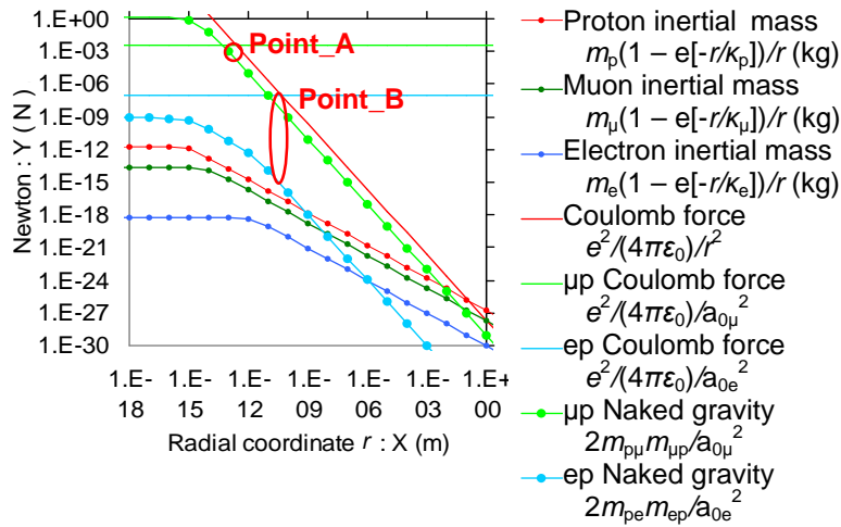
FIG. 3. The scalable inertial mass of fermions, and the Coulomb force and the naked gravity of a combination thereof. The red / green / blue dotted lines are the scalable inertial mass curves of each fermion. The solid lines are the line that Coulomb force. The Yellow-green / light-blue dotted lines (proton-muon, proton-electron) are the naked gravity line.
