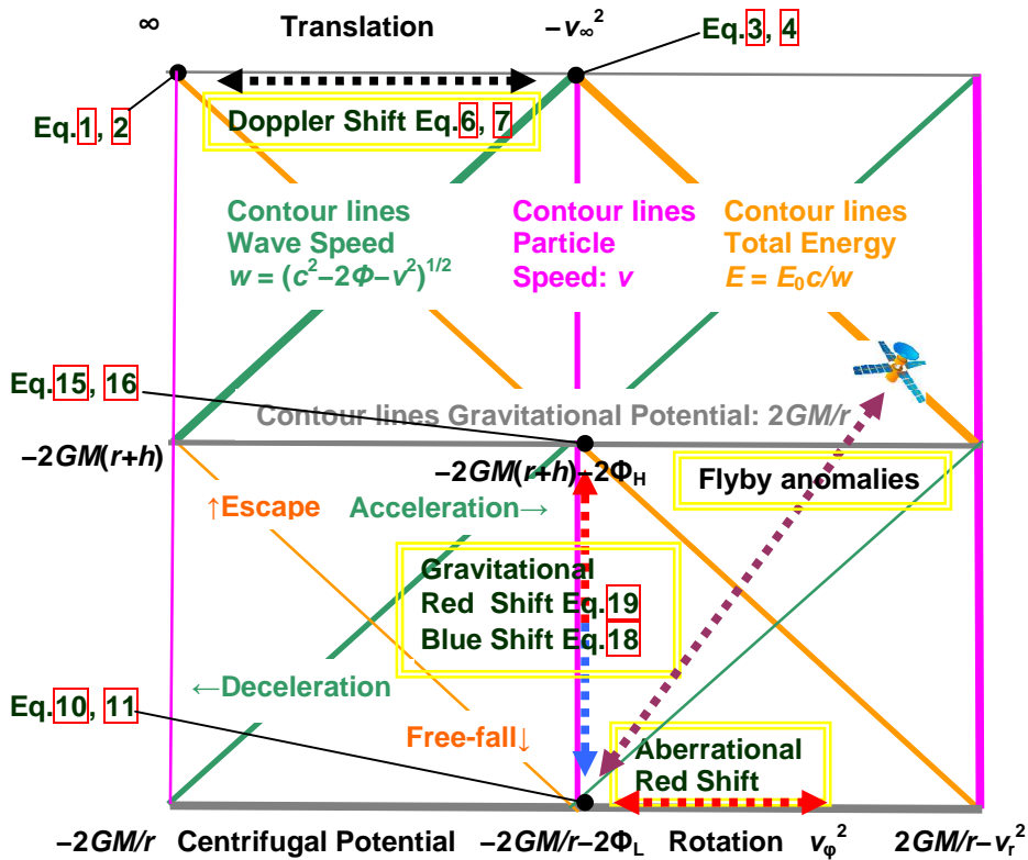
FIG.1. The frequency shift with the four-dimensional contour lines for the particle speed (Y axis), the gravitational potential (X axis), the total energy ( \ Clinoaxis) and the wave speed ( / Clinoaxis).
