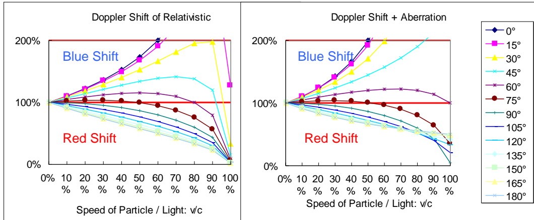
FIG.2: Comparison of the Doppler shift of this paper and the relativity: A Doppler shift of this paper is the same as almost the relativity at a relative speed ( v/c < 30\% ) of low-speed range or the transverse relative angle ( \theta = 90^\circ ). That aberration Doppler shift is smaller toward the longitudinal relative angle. It will have only the primary Doppler shift at the relative angle ( \theta = 0^\circ, 180^\circ ). On the other hand, the transverse Doppler shift of Relativistic occurs with the relative speed, and the relative angle is not involved, and the frequency will be shifted as disappear at the speed of light.
