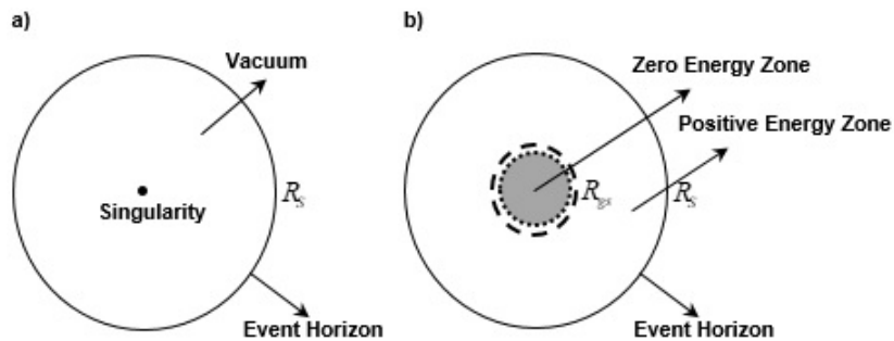
Figure 8: Internal structure of the black hole. a) Existing model b) New model. The black hole does not have a singularity in the center, but it has a zero energy zone.
