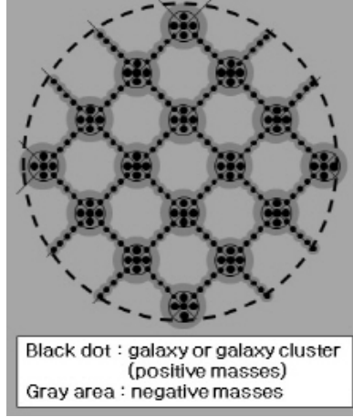
Figure 4: The current universe presumed in this model: Although the positive mass(black dot) constitute galaxy or cluster of galaxies and negative mass(gray) are almost evenly distributed in the entire universe, it is presumed that the density of negative mass(dark gray) near the galaxy would be higher than that of negative mass in the void area(gray), because negative mass receives attractive gravitational effect from large positive mass.
