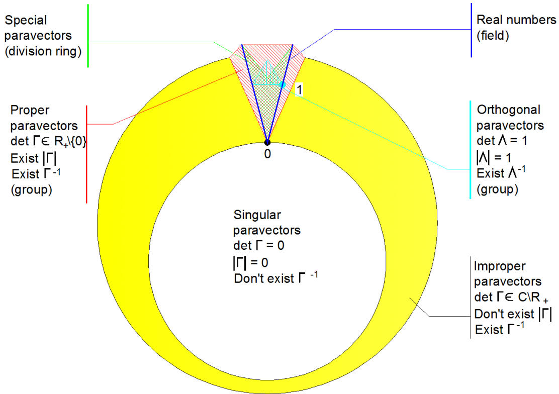
Figure 1: The ring of paravectors with some substructures
