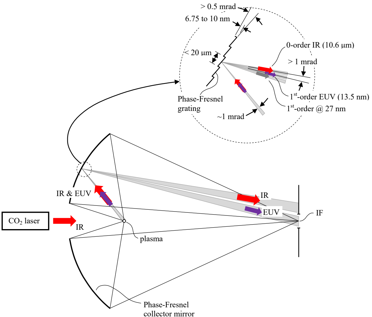
Figure 4. Phase-Fresnel-grating spectral filter.
