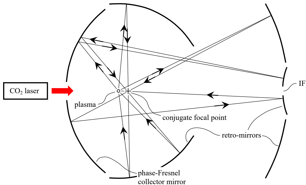
Figure 6. IR power recycling with relay imaging.
