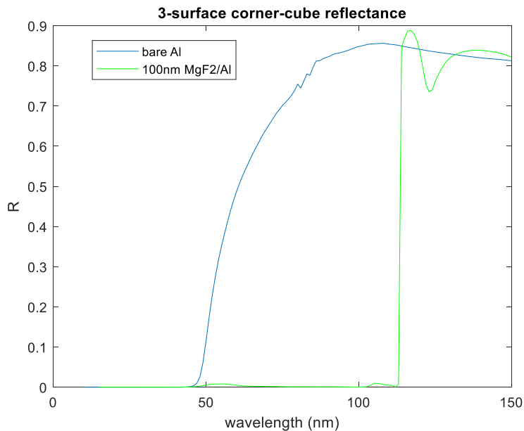
Figure 21. Corner-cube compound reflectance with bare or coated front-surface mirrors.
