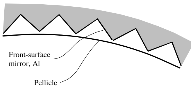
Figure 22. Bare-aluminum corner-cube reflector with pellicle.
