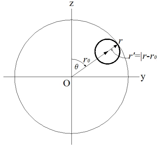
Fig. 1: A Euclidean sphere of radius r' centred at r=r_0 (Cartesian coordinates (x_0, y_0, z_0) at a distance r = r_0 = \sqrt{x_0^2 + y_0^2 + z_0^2} from the origin O; r and r_0 lying in the same radial line through O). Schwarzschild centred at the origin O but Hilbert, by setting the coefficient of (d\theta^2 + \sin^2\theta d\varphi^2) at r^2 , unwittingly centred at r_0 = \alpha = 2m (see Eq.(6.4)), mistakenly thinking he had centred at r=0 , thereby separating the sphere from its centre, misplacing its centre at r=0 . In other words, Hilbert unwittingly moved Schwarzschild's Euclidean sphere in Minkowski space to r=r_0 leaving its centre behind at r=0 . The large circle denotes a sphere relative to the origin of coordinates. The small circle denotes the sphere actually involved in Hilbert's solution. Thus, when r'=0 , r=r_0 , the latter misinterpreted as the radius of a black hole event horizon, with r=0 misinterpreted as an infinitely dense 'physical' singularity of a black hole, where spacetime curvature is 'infinite'*. Note that as r' grows its sphere engulfs the origin O and beyond, so none of Euclidean 3-space is left out. Cosmology however, seeks to stop at r=0 , all the while attempting to drive the centre of the sphere r' down to r=0 when in fact it is at r_0 = \alpha = 2m . When r=0 in Hilbert's solution, the radius r' = r = r_0 = \sqrt{x_0^2 + y_0^2 + z_0^2} and the centre of the sphere at (x_0, y_0, z_0) , as Eq.(6.5) attests. Hilbert confounded the origin of the coordinate system for the centre of the Euclidean sphere, and so his solution is invalid.
