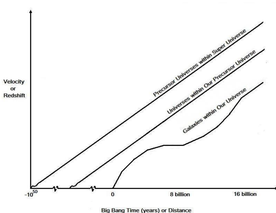
FIG. 10. Hubble's law.
